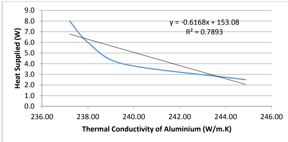
Figure 4: Graph of Heat Supplied against Thermal Conductivity of Aluminium
