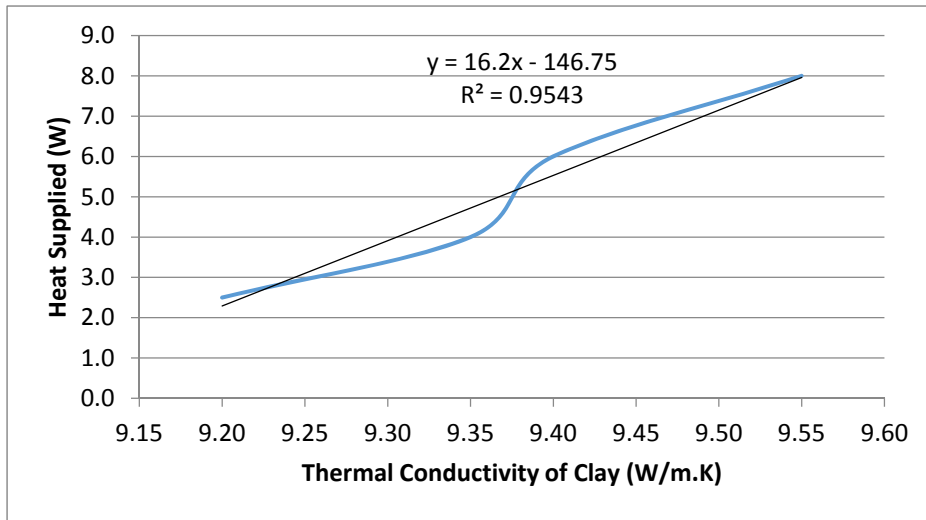
Figure 7: Graph of Heat Supplied against Thermal Conductivity of Clay
