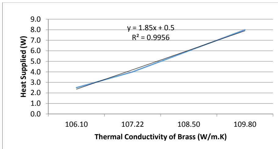
Figure 3: Graph of Heat Supplied against Thermal Conductivity of Brass
