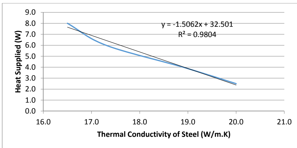
Figure 5: Graph of Heat Supplied against Thermal Conductivity of Steel
