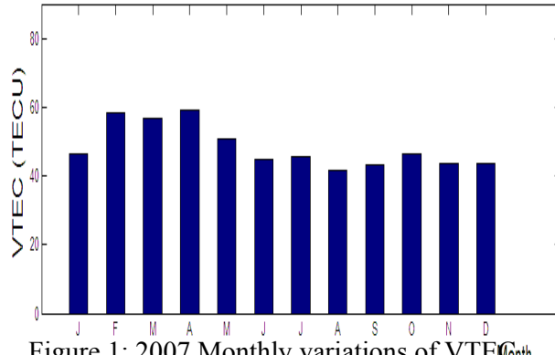
Figure 1: 2007 Monthly variations of VTEC
