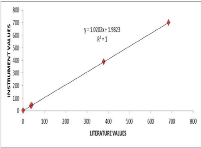
164 165 166 Figure 6.0: Plot between Measured viscosity values and literature values 167
