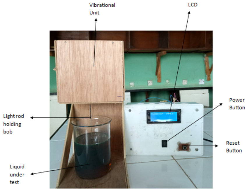
Figure 2: Image of the developed viscometer
