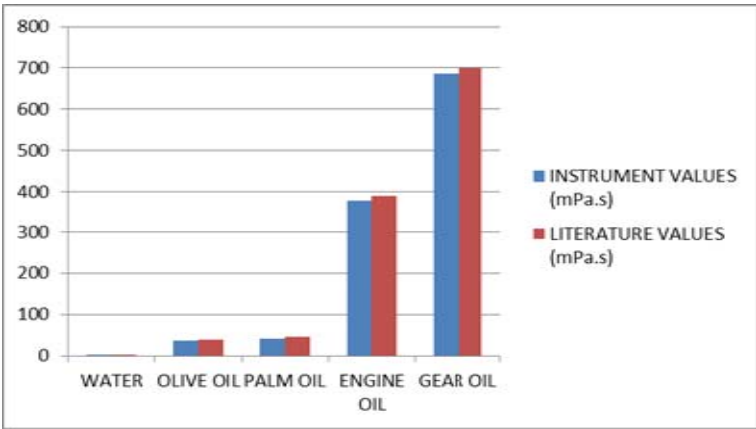
170 171 Figure 7.0: Bar chart between the measured viscosity values and literature values 172
