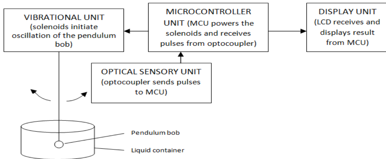
Figure 3: Operational chart of the developed viscometer
