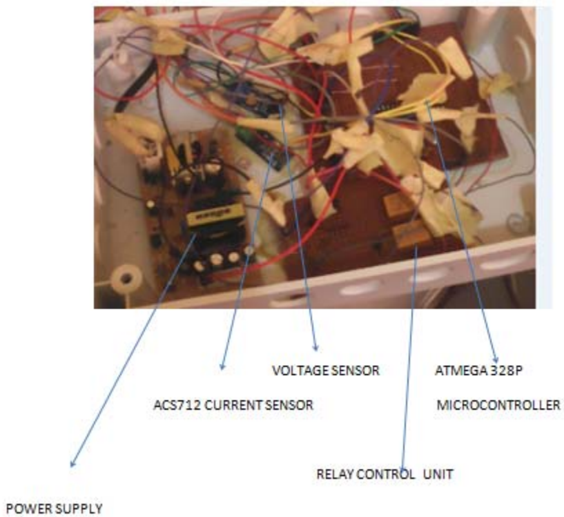
Figure 1b: Image of the developed instrument showing the circuit components
