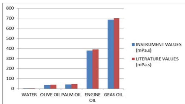
Figure 7.0: Bar chart between the measured viscosity values and literature values
