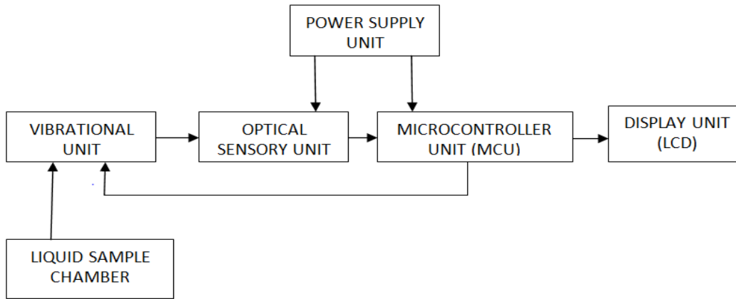
Figure 1a: Block diagram of the developed viscometer
