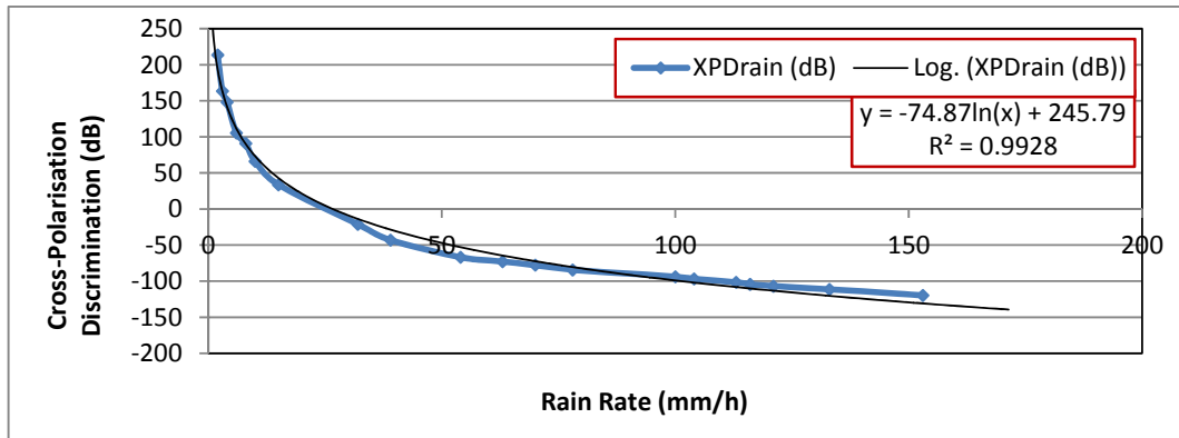
Fig. 7. Variation of Cross polarization discrimination (XPD) with rain rate
