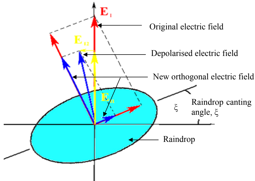
Figure 3: Depolarization of signal E_1 , through an oblate shaped raindrop [8].
