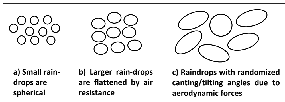
Figure 2: Variation in raindrop size, shape and angle during rain events [6]
