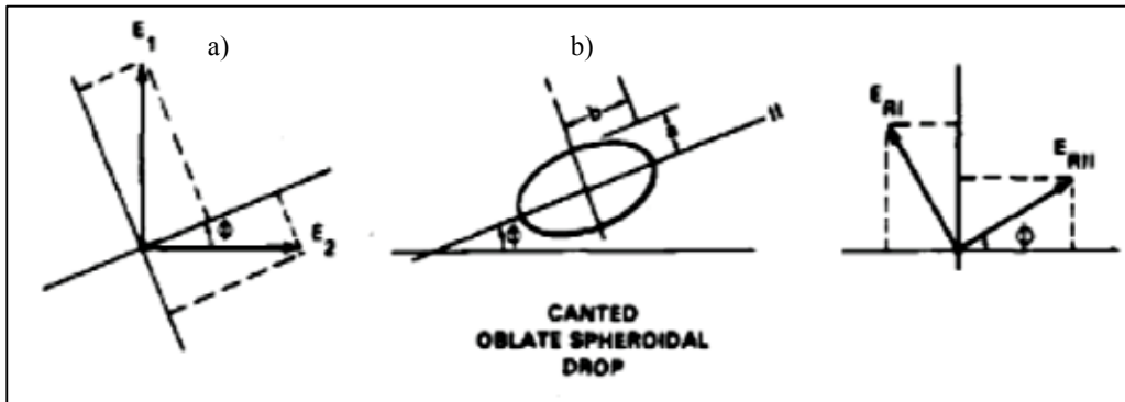
Figure 1: Canting effect of deformed raindrop [10]: Vector relationship for a depolarizing medium. (a) Co- and cross-polarized waves for linear transmission and (b) Classical model for a canted oblate spherical rain drop.
