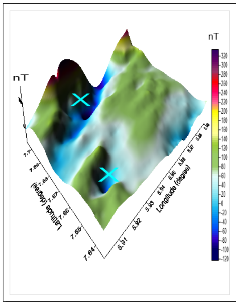
Figure 7: 3D image map of AkunnuAkoko area.
