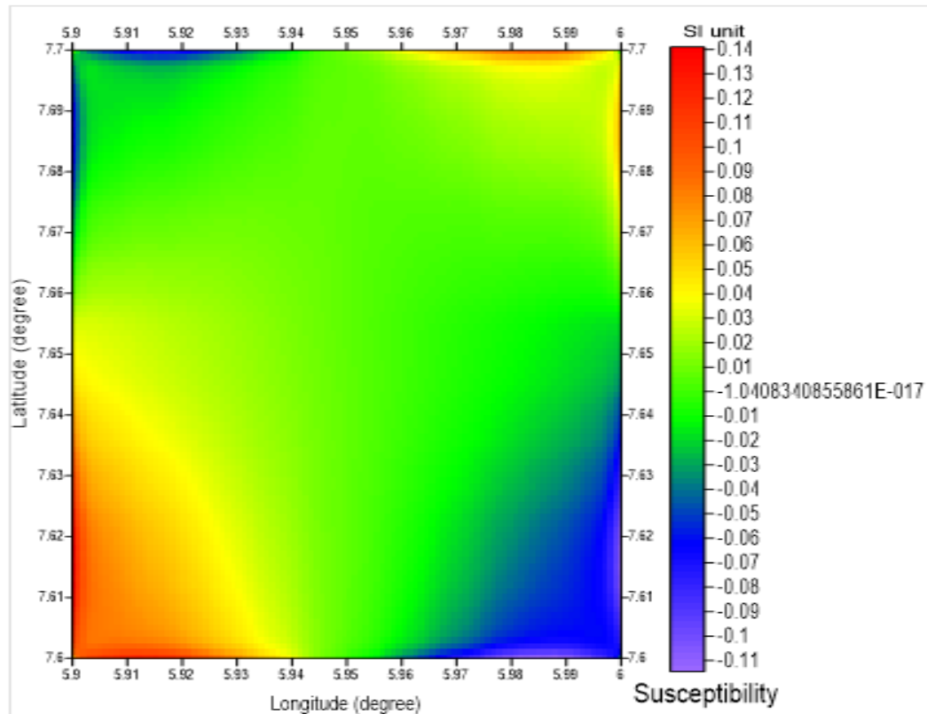
Figure 8: Susceptibility map of Akunnu Akoko area.
