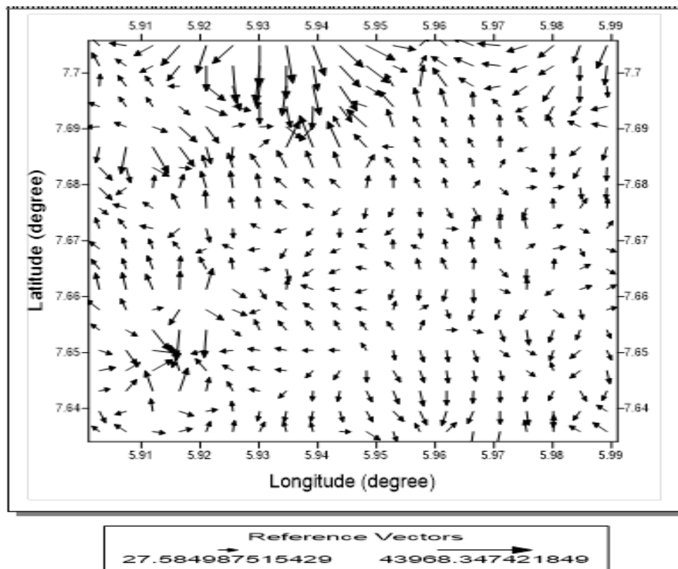
Figure 6: Vector map of AkunnuAkoko area.
