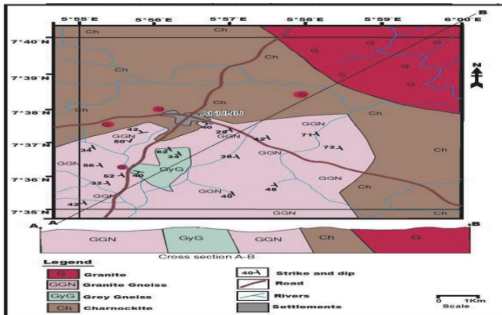
Figure 2: Geology of Akunnu Area [10].
