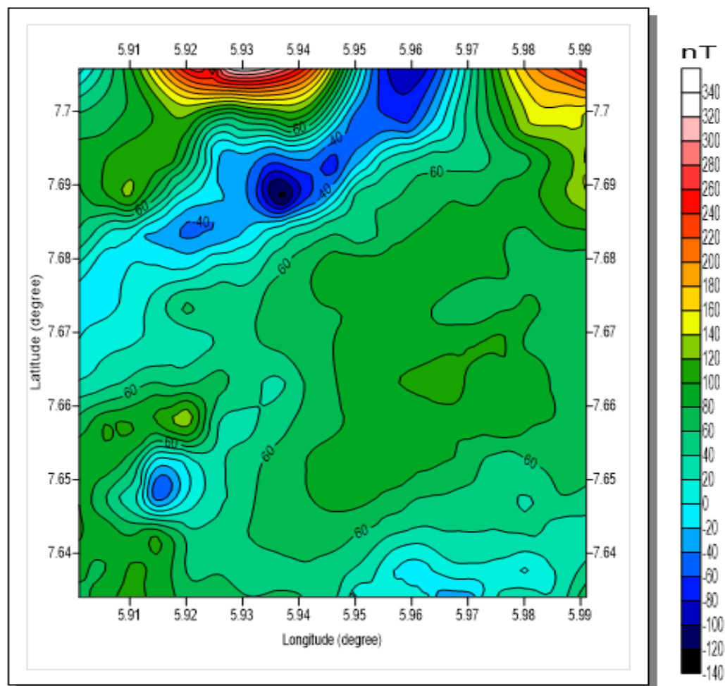
Figure 5: Contour map of Akunnu Akoko area with contour interval 20 nT.
