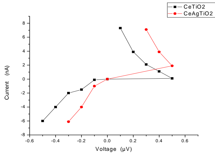
Figure 3: Comparison of I-V curve by CSAFM technique for CeTiO 2 and CeAgTiO 2 .
