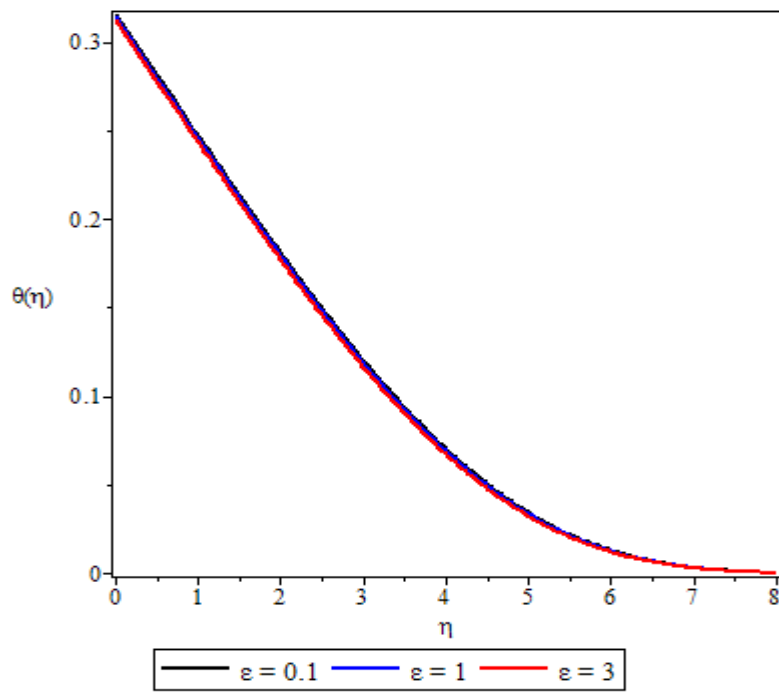
Fig.4.8 temperature profile for \varepsilon
