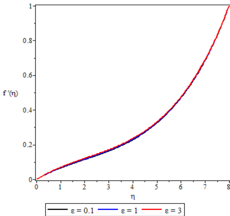
Fig. 4.7 velocity profile for \epsilon
