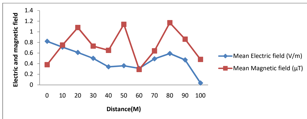
Fig.2: Plot of Electric and Magnetic Field Strength around 11kVA Line
