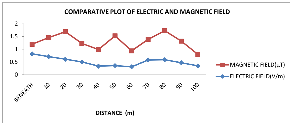
Fig.3: Plot of Electric and Magnetic Fields strength around 33kVA power line
