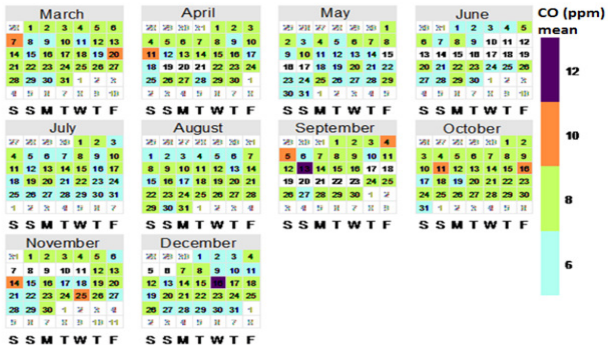
Figure 4(a): Calendar plot for CO concentration in 2009 with a user-defined categorical scale.
