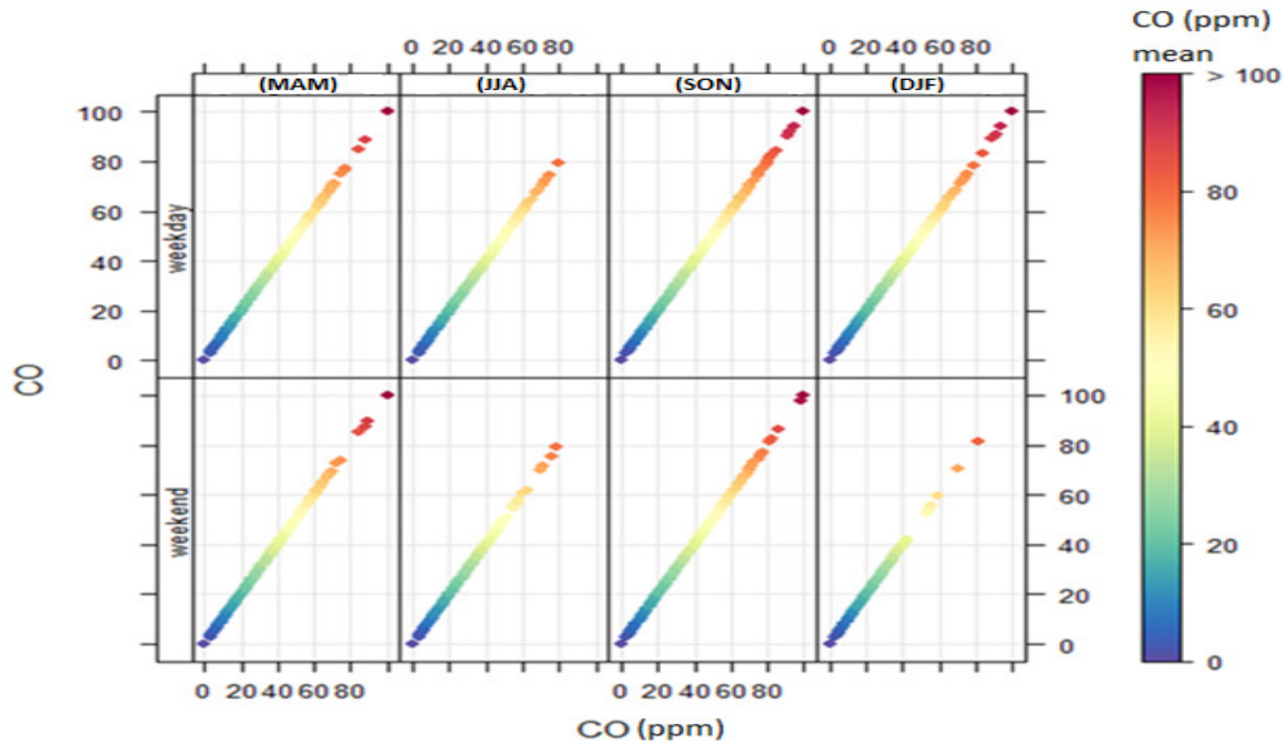
Figure 5: Comparison between Weekdays and Weekends CO concentration for 15 minutes exposure by different level Split by Season
