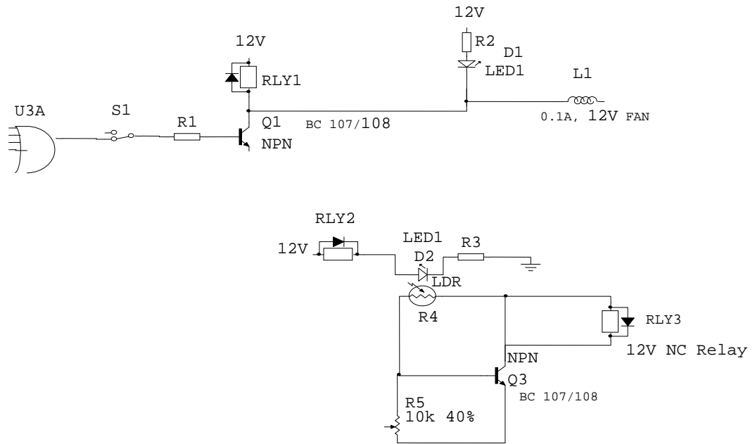
Fig.9 Control circuit for Automatic Fire Suppression system
