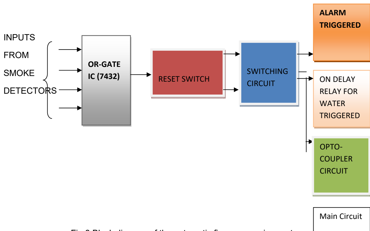
Fig.8 Block diagram of the automatic fire suppression system
