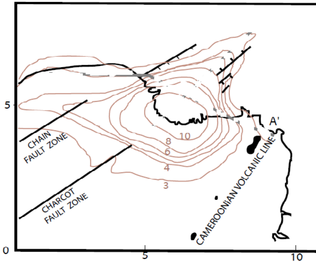
Fig. 13: Isopach map of the Niger Delta Sedimentary Basin (Modified from [28]).
