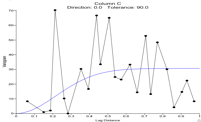
231 232 Fig. 8: Computed variogram and variogram model for geothermal gradient.
