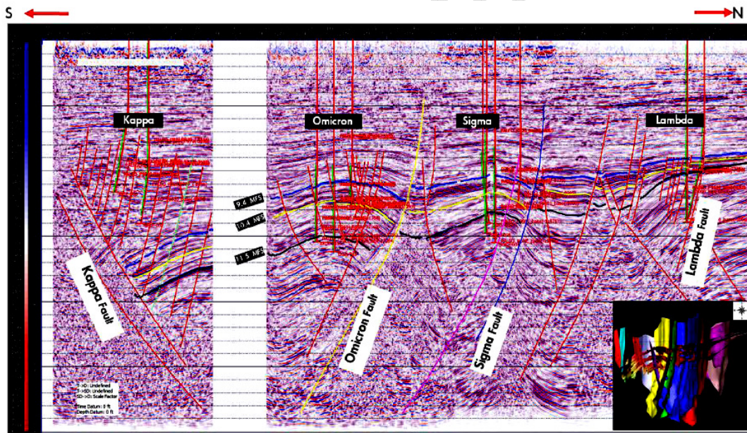
Fig.12: Seismic data from part of the study area with complex fault structures
