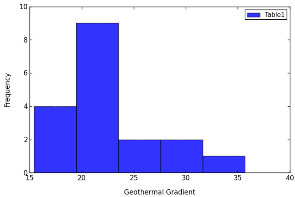
Fig.6: Histogram of the Geothermal Gradient (°C/Km)
