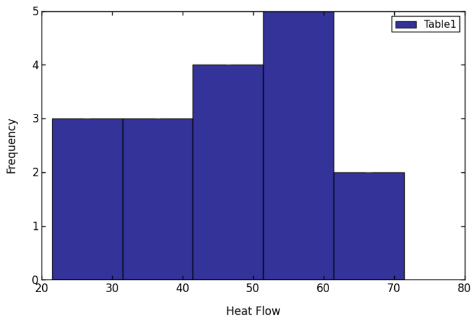
Fig.7: Histogram of the Heat Flow (mW/m 2 )
