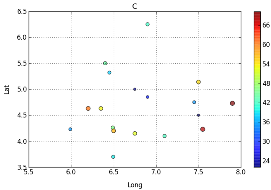
189 Fig. 4: Base Map of the Study Area Showing the Heat Flow Values ( \text{mW/m}^2 )
