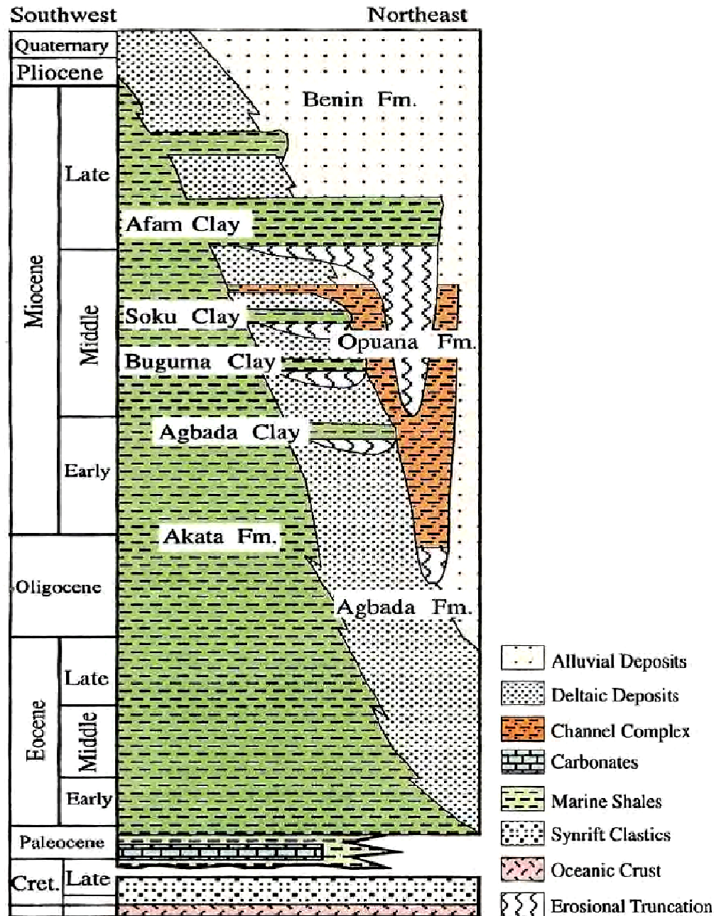
Fig. 2: Lithostratigraphy of the Niger Delta
