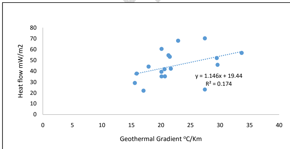
Fig. 5: A plot of heat flow against geothermal gradient
