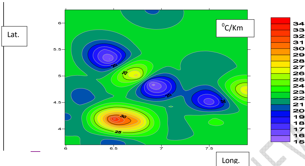
Fig. 10. Geothermal gradient map calculated using ordinary kriging algorithm
