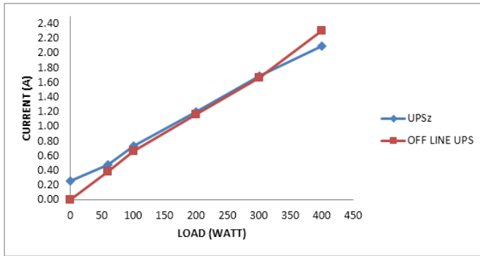
Fig 27: A graph of load against current for both the UPSz and the offline UPS at 180V AC input voltage.
