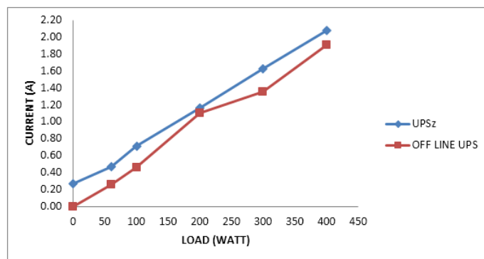
Fig 25: A graph of load against current for both the UPSz and the offline UPS at 220V AC input voltage.
