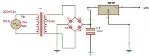
Fig 5. Circuit diagram of the Rectifier K2 with transformer T_1
