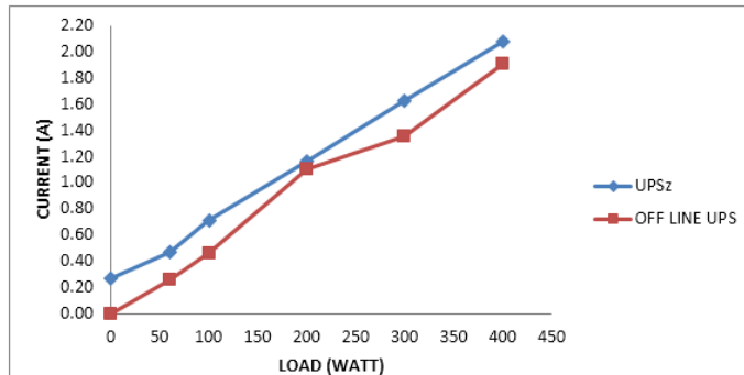
Fig 25: A graph of load against current for both the UPSz and the offline UPS at 220V AC input voltage.
