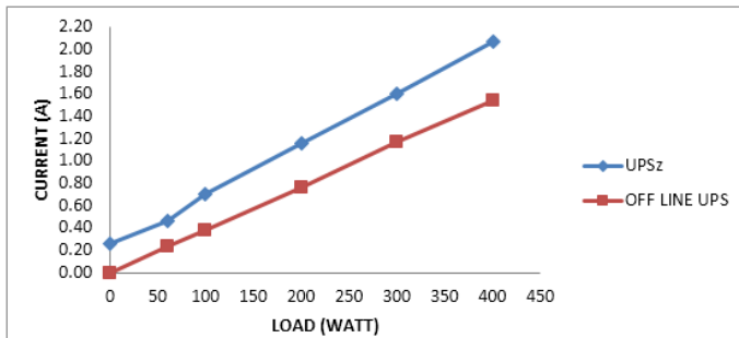
Fig 23: A graph of load against current for both the UPSz and the offline UPS at 260V AC input voltage.
