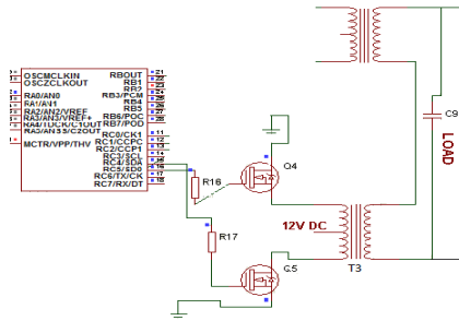
Fig 7: circuit diagram of the standby DC-AC converter interfacing the transformer T_3
