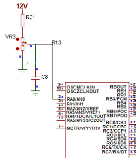
Fig 8: The low battery circuit interfacing with the microcontroller
