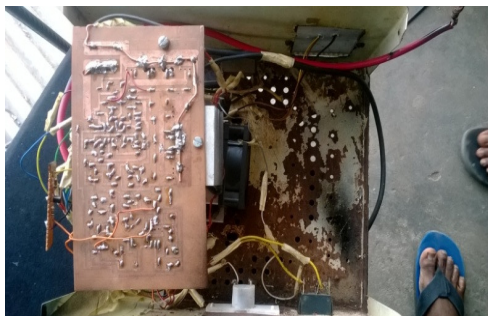
Fig 19: packaging of the UPSz into a casing.
