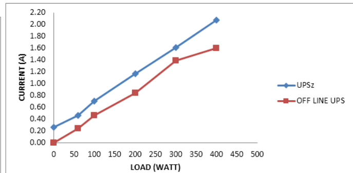
Fig 24: A graph of load against current for both the UPSz and the offline UPS at 240V AC input voltage.
