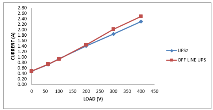
Fig 30: A graph of load against current for both the UPSz and the offline UPS during mode II
