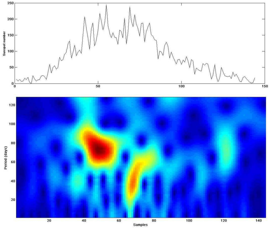
Fig. 6. CWT of Solar Cycle 23 using a Morlet Wavelet of size 8 and 128 voices. In figure X axis represents the number of samples and Y axis represents scale. The upper panel shows the raw data of the time series and lower panel its continuous wavelet transform (CWT).
