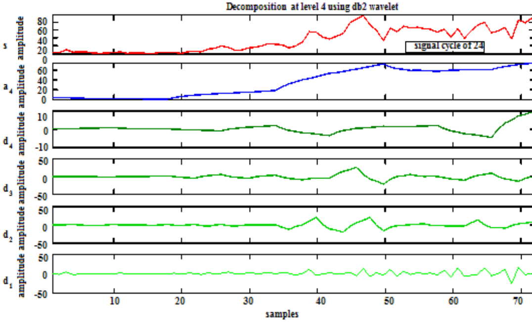
Fig. 3. DWT decompositions of Solar Cycle 24 using Daubechies2 wavelet. Anomalous variation showing between 40 to 50 no. of samples (i.e. at the maximum phase of cycle).
