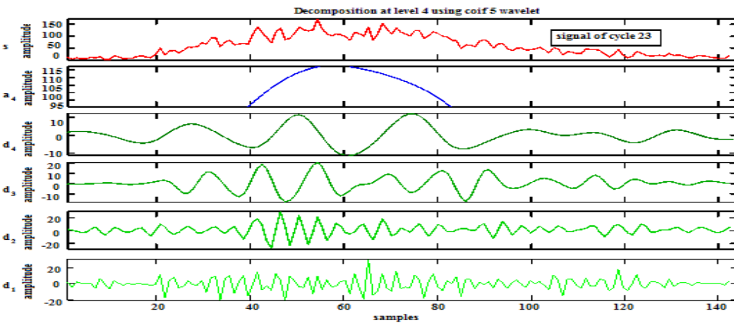
Fig. 2. DWT decompositions of Solar Cycle 23 using Coifman5 wavelet. Anomalous sharp variation should be found between 40-60 no. of samples (i.e. at the maximum phase of cycle).
