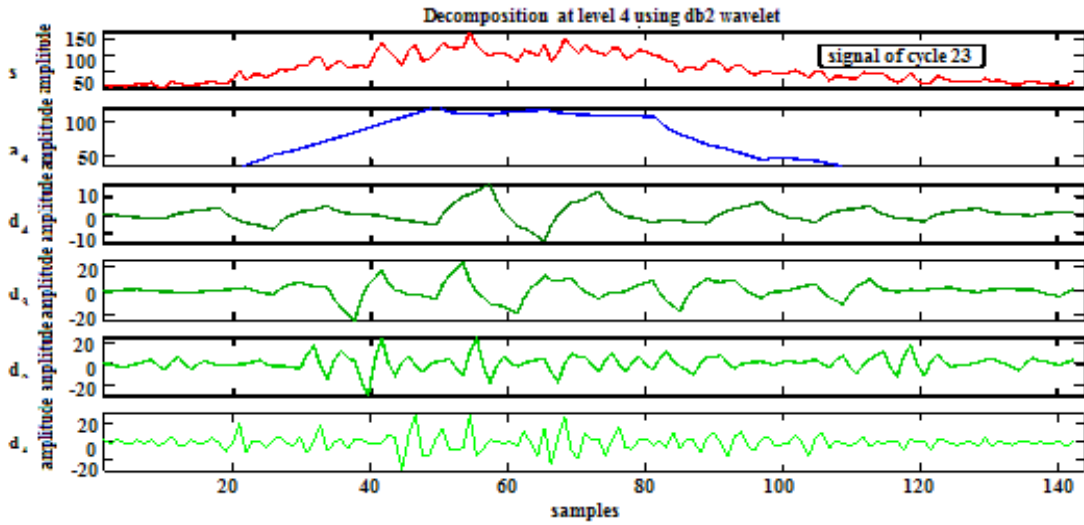
Fig. 1. DWT decompositions of Solar Cycle 23 using Daubechies2 wavelet. Anomalous variation should be found between 45-60 no. of samples (i.e. at the maximum phase of cycle).
