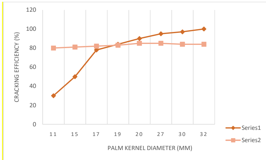
Fig. 1: Graph of Cracking Efficiency (%) vs Palm Kernel Diameter (mm) (Where Series 1 is the efficiency of the existing Machine and Series 2 is the efficiency of the developed Machine)
