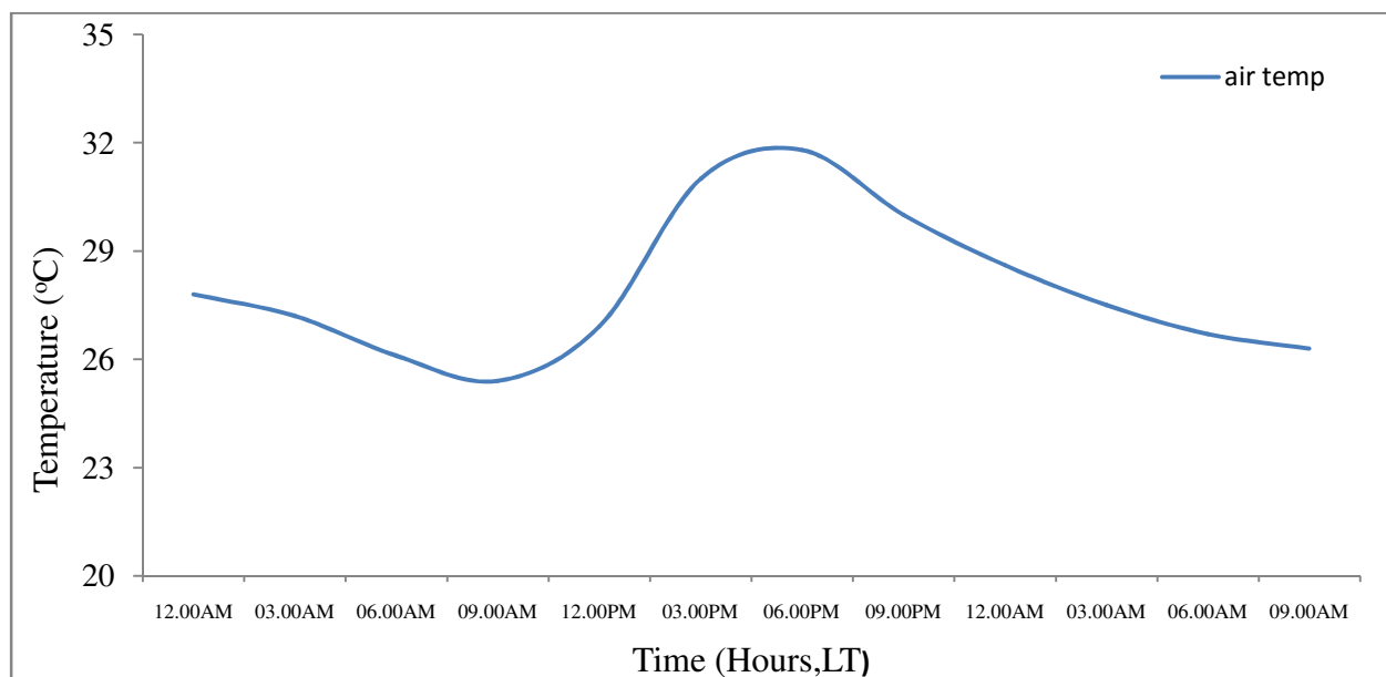
Figure 1: Diurnal variation of air temperature between the 23 rd and 24th December, 2011, for Ministry of Agriculture, Akure during the dry season.
