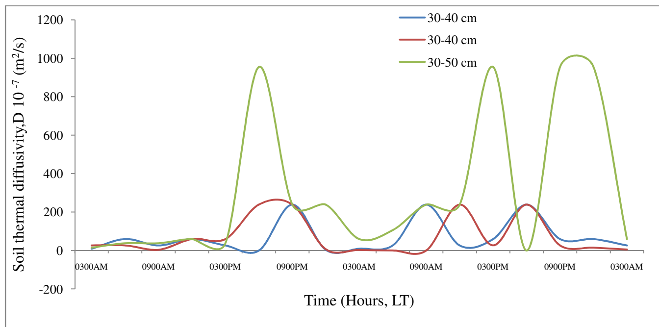
Figure 6: A typical plot of diurnal variation of the thermal diffusivity for Ministry of Agric, Akure South, during the wet season (10 th and 11th of May, 2012).
