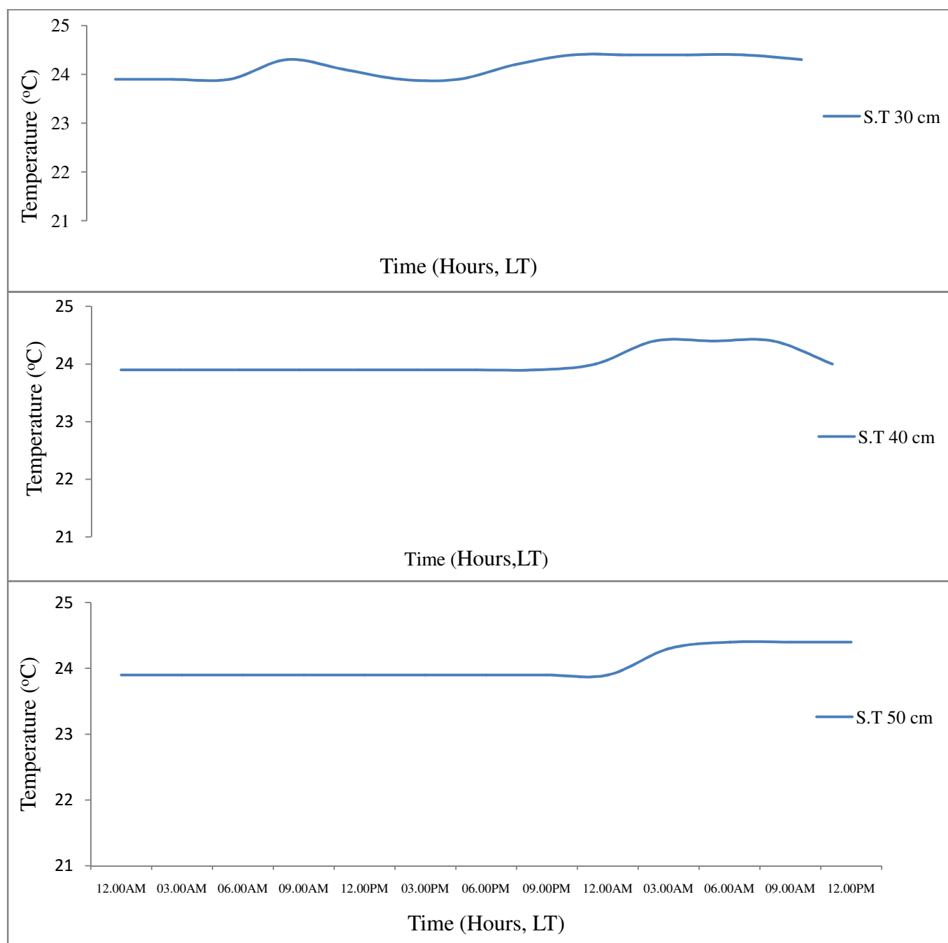
Figure 3: Diurnal variation of soil temperature between the 23th to 24th, December, 2011 at Ministry of Agriculture, Akure during the dry season.
