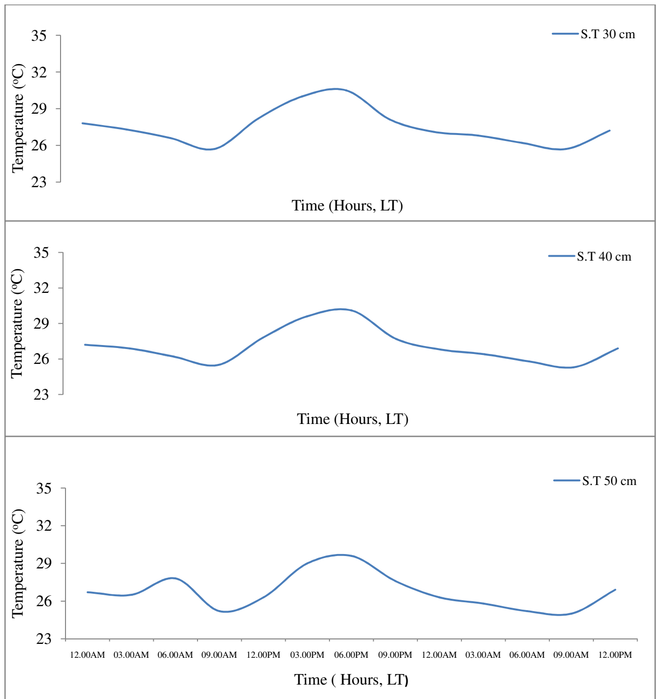
Figure 4: Diurnal variation of soil temperature between the 10th and 11th May, 2012, at Ministry of Agriculture, Akure during the wet season.
