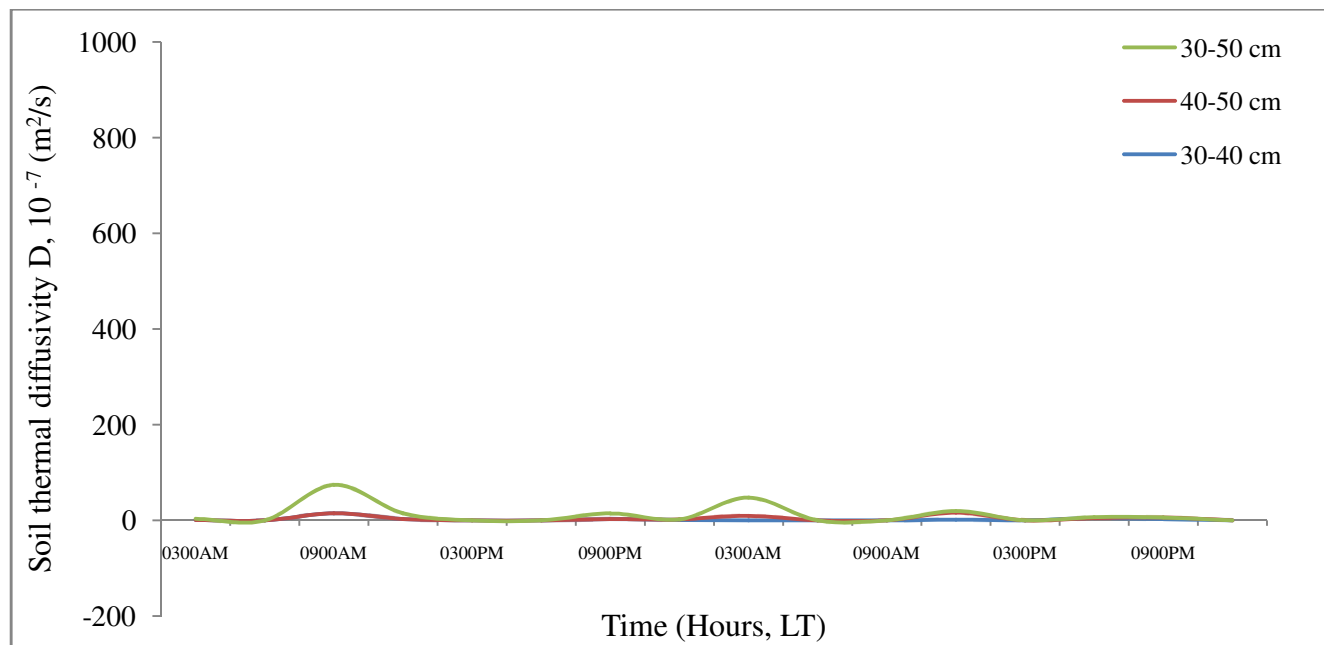
Figure 5: A typical plot of diurnal variation of thermal diffusivity for Ministry of Agriculture, Akure South, during the dry season (23 rd and 24 th of December, 2011).
