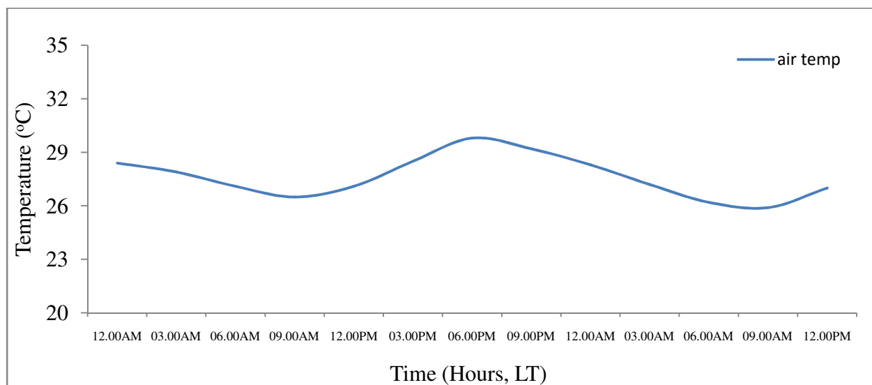
Figure 2: Diurnal variation of air temperature between the 10 th and 11th May, 2012, at Ministry of Agriculture, Akure during the wet season.
