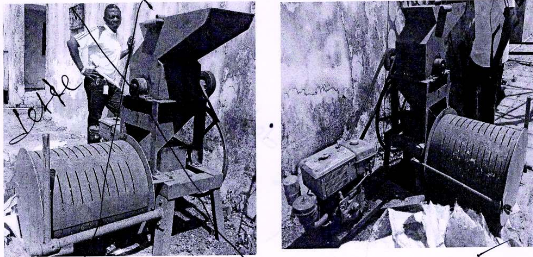
Fig 15: Picture of the Fabricated Palm Kernel Shelling Machine
