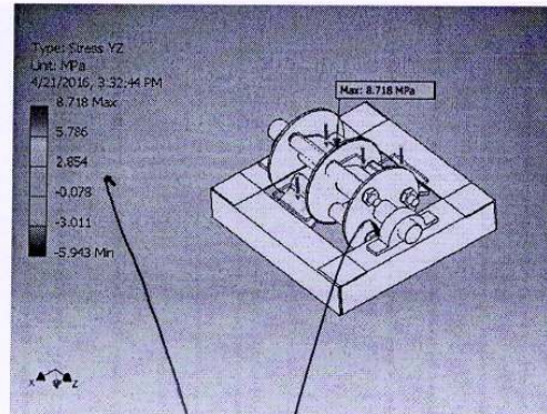
Fig. 10: Stress YZ analysis of the Hammer Mill
