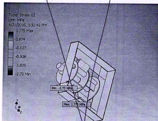
Fig. 8: Stress XZ analysis of the Hammer Mill
