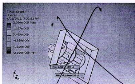
Fig. 4: Strain YY analysis of the Hammer Mill
