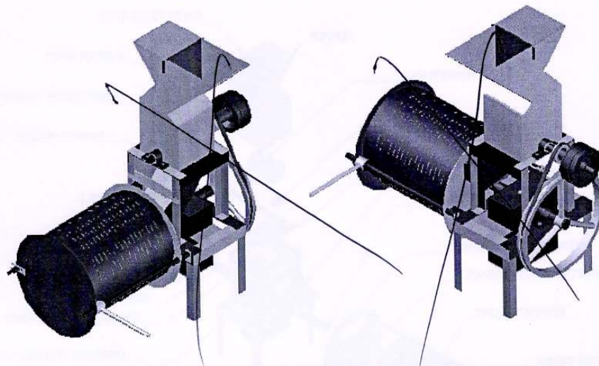
Fig 18: 3D CAD Views of the Modeled Palm Kernel Shelling Machine
