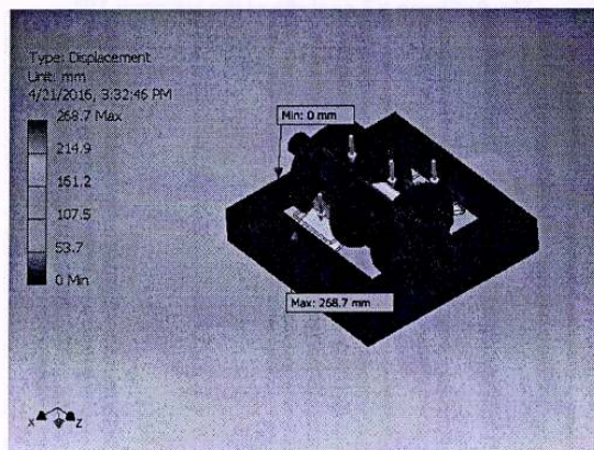
Fig. 6: Displacement analysis of the Hammer Mill
