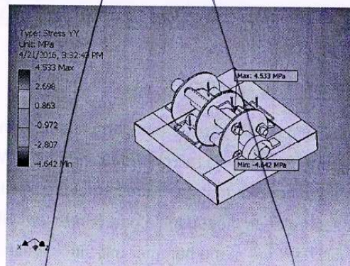
Fig. 12: Stress YY analysis of the Hammer Mill
