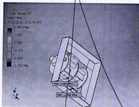
Fig. 9: Stress XY analysis of the Hammer Mill
