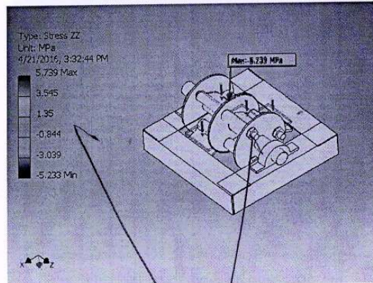
Fig. 13: Stress ZZ analysis of the Hammer Mill
