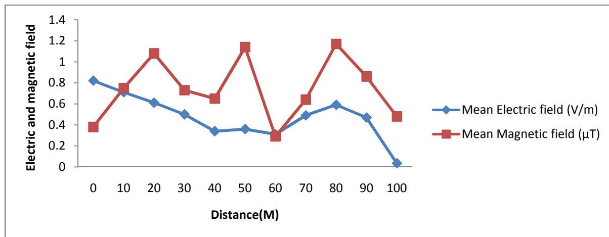
Fig. 3: Plot of Electric and Magnetic Field Strength around 11KVA Line
