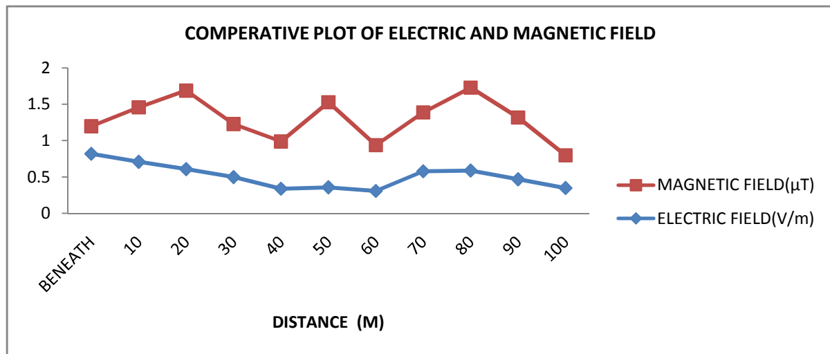
Fig. 4: Plot of Electric and Magnetic Fields strength around 33kVA power line
