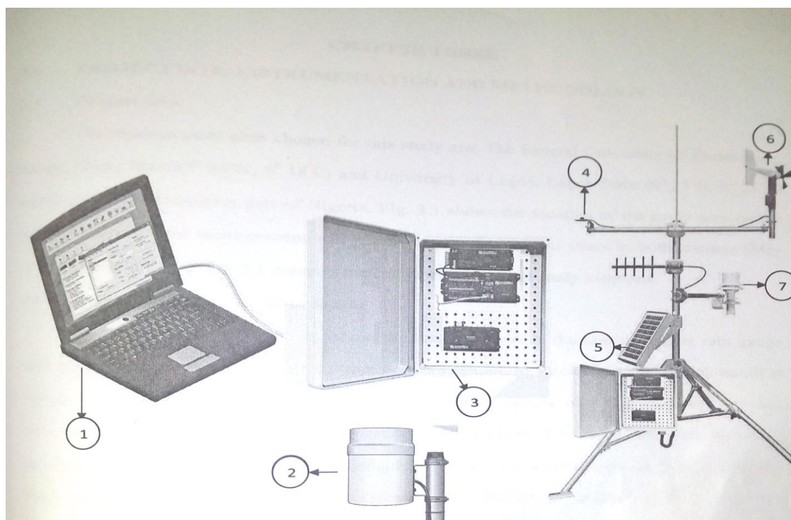
Fig. 3. A typical tropospheric data acquisition system components. Key: (1) Laptop, (2) Tipping bucket rain gauge, (3) CR100 data logger unit, (4) Pyranometer, (5) Solar panel, (6) Wind vane; and (7) Radiation shield.
