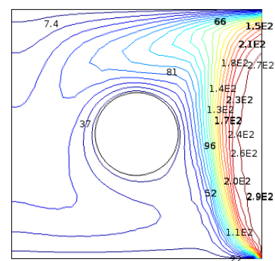
Fig.3.Isotherms (a) & Streamlines (b) in the cavity for various Pr and Ha = 60, Ra = 10^5, \phi = 0^\circ .
