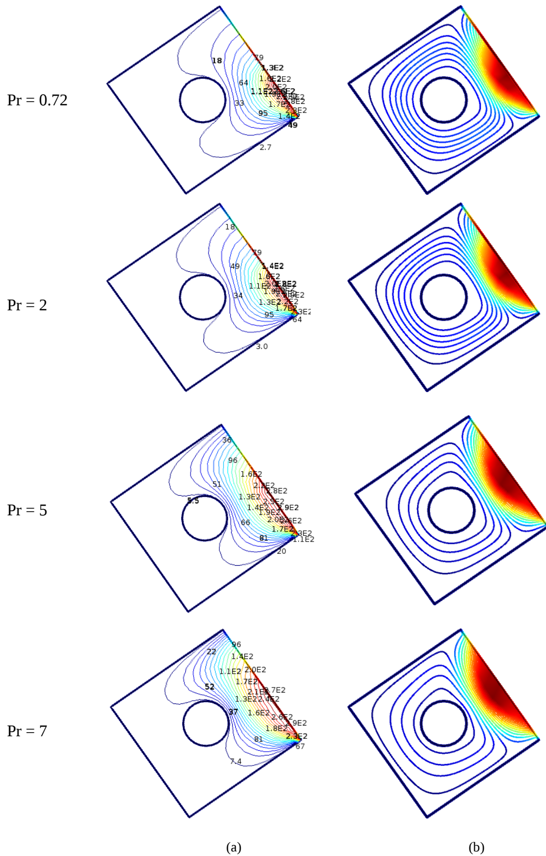
Fig. 6. Isotherms (a) & Streamlines (b) for various Pr while Ha = 60, Ra = 10^4, \phi = 35^\circ in the cavity .
