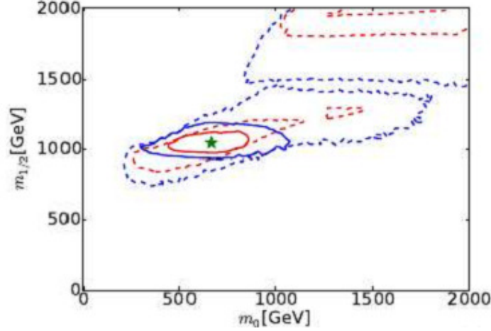
Fig. 3. The m_0 , m_{1/2} planes in the CMSSM from [6].
