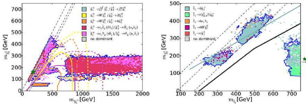
Fig. 5. Left panel: the (m_{\tilde{\chi}_1^\pm}, m_{\tilde{\chi}_1^0}) plane with 68% and 95% CL contours shown as solid red and blue lines, respectively. The coloured shadings indicate where the corresponding branching ratios exceed 50%. Right panel: the (m_{\tilde{t}_1}, m_{\tilde{\chi}_1^\pm}) plane with 68% and 95% CL contours shown as solid red and blue lines, respectively, as well as colored regions where the indicated branching ratios exceed 50% [10].
