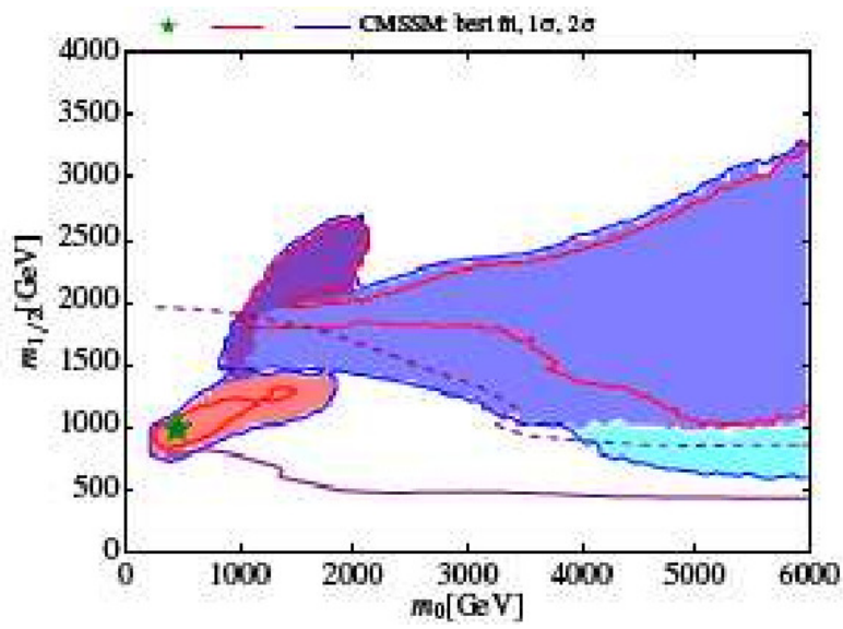
Fig. 1. The m_0 , m_{1/2} planes in the CMSSM from [4].
