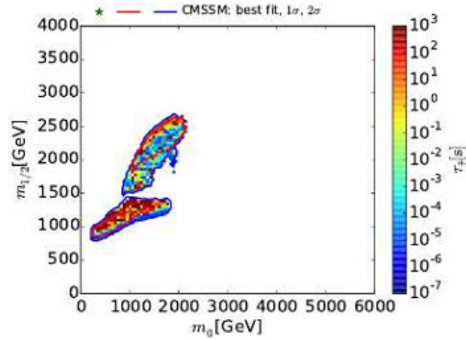
Fig. 3. The m_0 , m_{1/2} planes in the CMSSM from [6].
