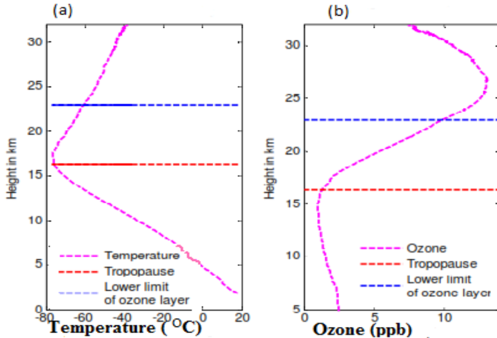
Figure 3: Mean Vertical variation; (a) temperature, (b) Ozone over Nairobi 2010 to 2015
