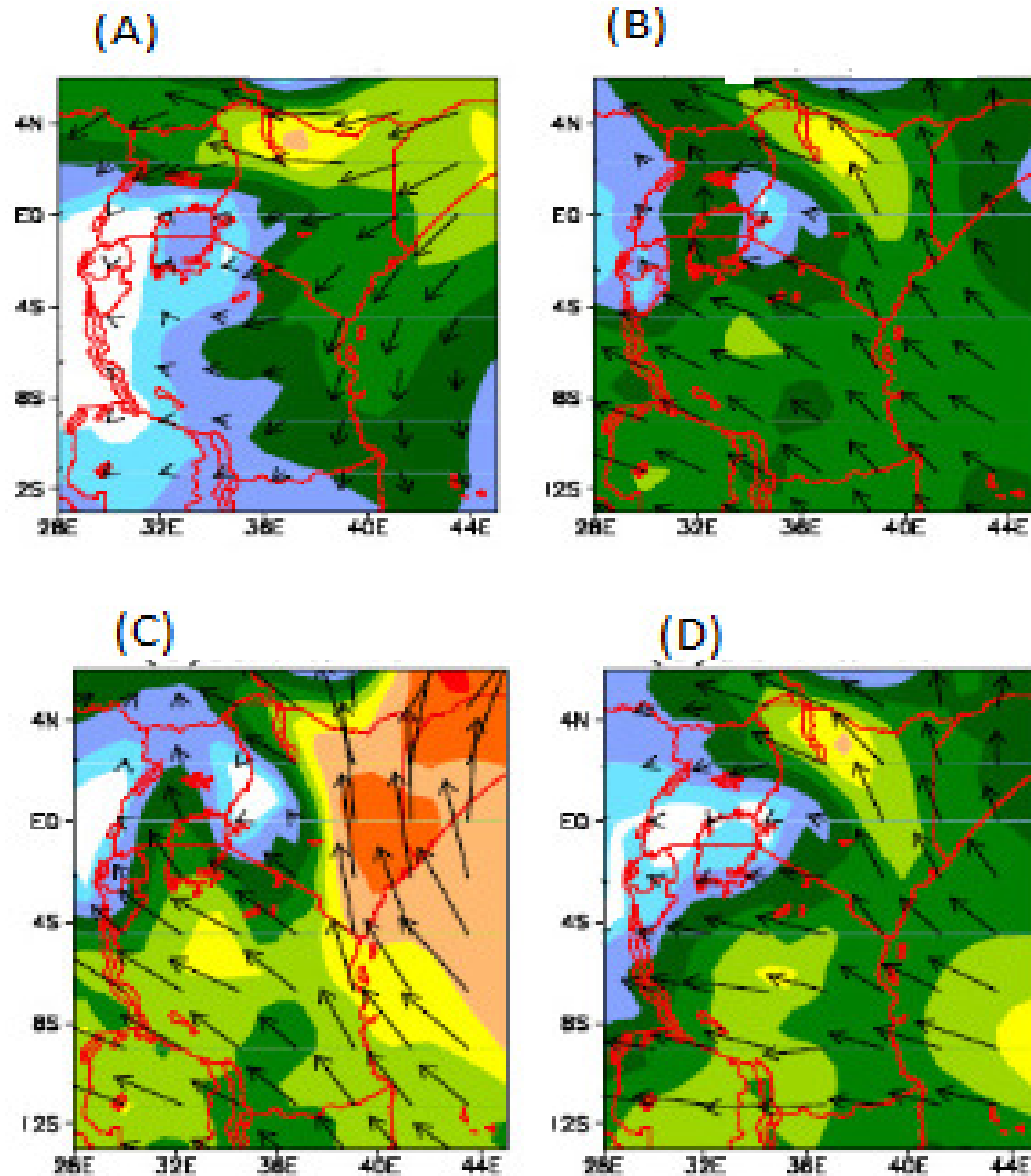
Figure 6: The mean seasonal wind speed (m/s) and direction (a) December, January and February (DJF) (b) March, April and May (MAM) (c) June, July and August(JJA) (d) September, October and November (SON)
