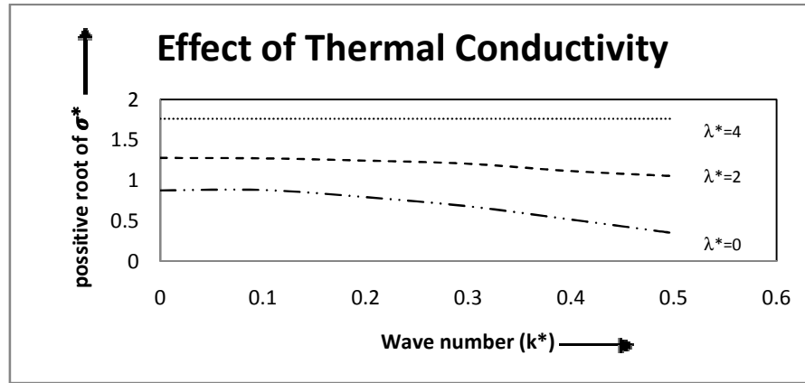
Fig. 1. The growth rate of instability is plotted against the dimensionless wave number k^* with variation in the thermal conductivity \lambda^* = 0, 2, 4 , with taking the values of k_s^*, \vartheta^*, V^*, k_1^*, \mathcal{Q}^* and \tau^* as unity.
