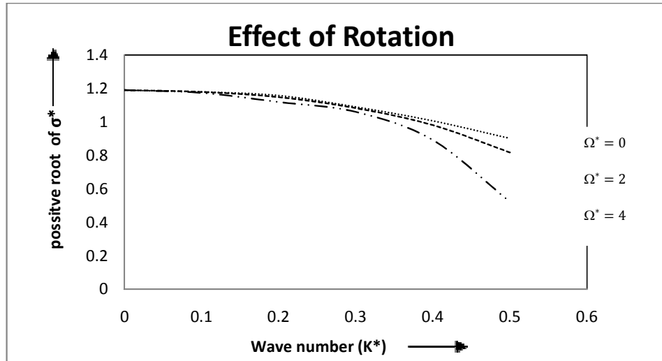
Fig. 6. The growth rate of instability is plotted against the dimensionless wave number k^* with variation in the rotation \Omega^* = 0, 2, 4 , with taking the values of k_1^* , k_s^* , \vartheta^* and \tau^* as unity.
