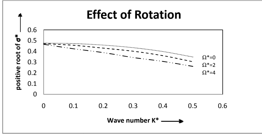
Fig. 3. The growth rate of instability is plotted against the dimensionless wave number k^* with variation in the Rotation \Omega^* = 0, 2, 4 , with taking the values of \lambda^*, V^*, k_s^*, \vartheta^*, k_1^* and \tau^* as unity.
