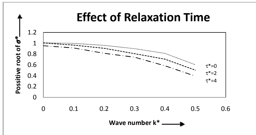
Fig. 4. The growth rate of instability is plotted against the dimensionless wave number k^* with variation in the relaxation time \tau^* = 0, 2, 4 , with taking the values of k_s^*, k_1^*, \Omega^* , and \vartheta^* as unity.
