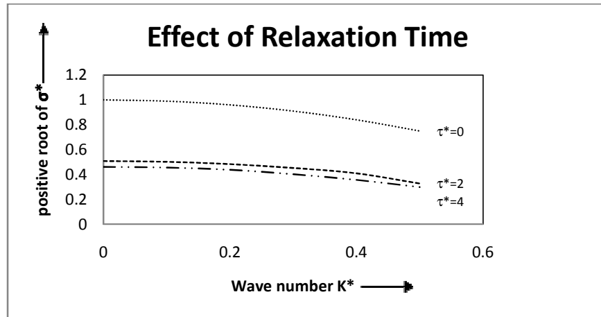
Fig. 2. The growth rate of instability is plotted against the dimensionless wave number k^* with variation in the relaxation time \tau^* = 0, 2, 4 , with taking the values of k_s^*, V^*, \vartheta^*, k_1^*, \mathcal{Q}^* and \lambda^* as unity.
