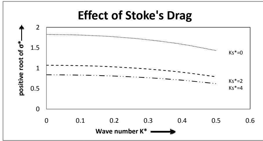
Fig. 5. The growth rate of instability is plotted against the dimensionless wave number k^* with variation in the Stokes' drag constant k_s^* = 0, 2, 4 , with taking the values of k_1^* , \Omega^* , \vartheta^* and \tau^* as unity.
