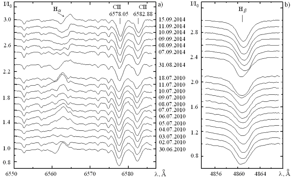
Figure 1. Profiles of the H \alpha and H \beta lines in the spectra of HD198478 observed in 2010 and 2014.
