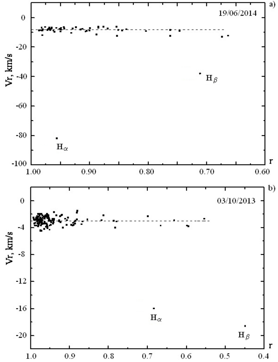
Figure 3. Kinematic slices: a) for HD198478 and b) for HD187982
