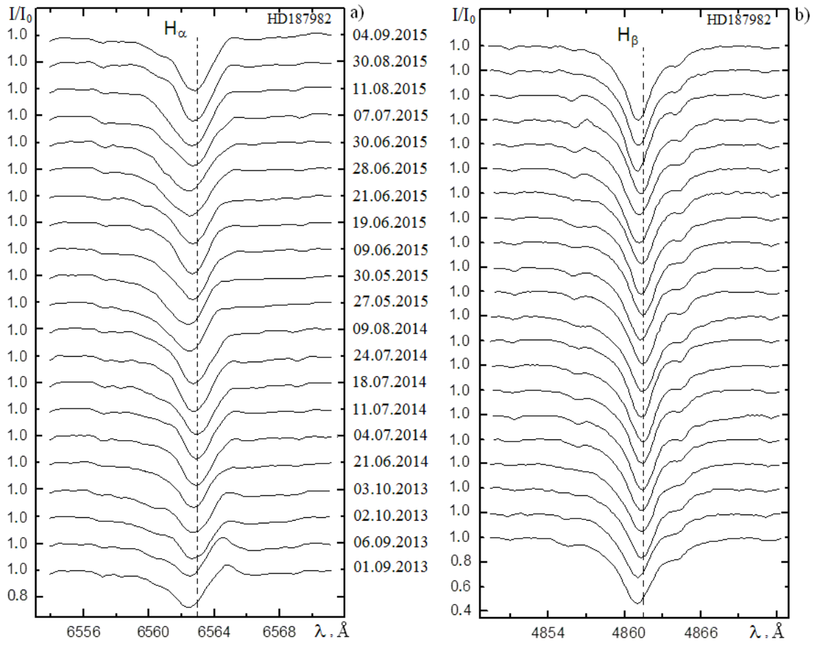
Figure 2. Profiles of the H \alpha and H \beta lines in the spectra of the star HD187982 observed in 2013-2015.
