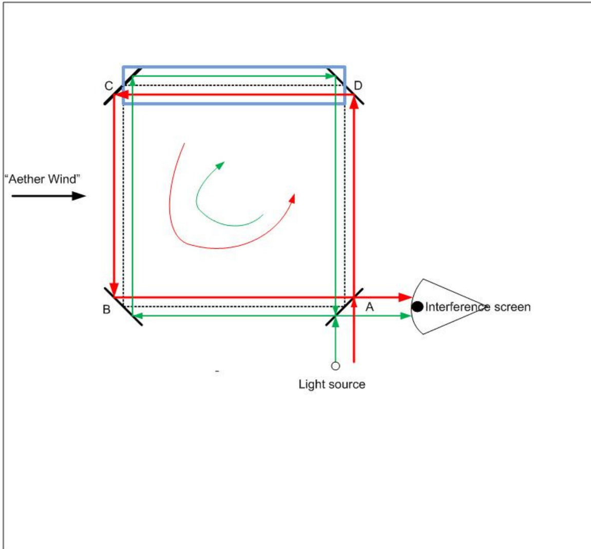
Fig. 1 Instrument motion with shielded arm moving parallel to the “aether wind” The light source as well as the screen where interference occurs between the two light beams is located in point “A”. Also, a half-silvered mirror is used as a light splitter.
