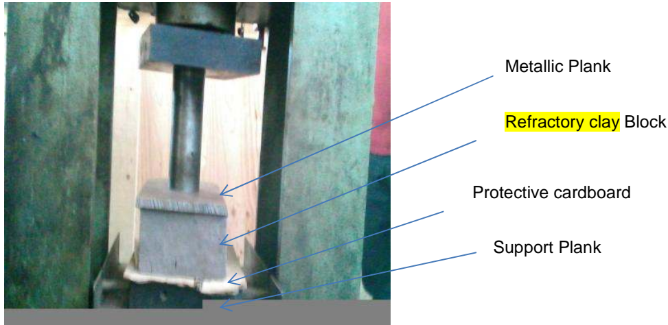
Figure 1 : Measuring Compressive Strength
