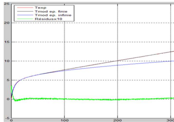
Figure 12: Curve experimental model and testing of residues on the sample 10 BTC..
