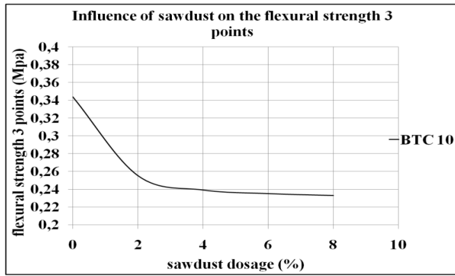
Figure 6: Influence of dosage of Afzelia sawdust on the resistance in three points flexion
