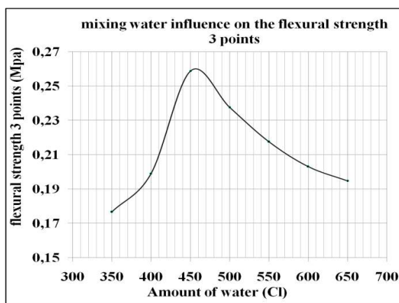
Figure 9: Influence of wasting water on the resistance in flexion three points
