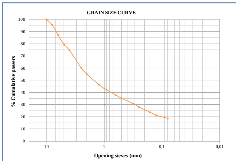
Figure 2 : Grading curve of the laterite
