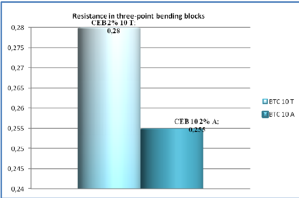
Figure 10: Resistance in flexion three points and in compression with Afzelia africana and Tectona grandis sawdusts
