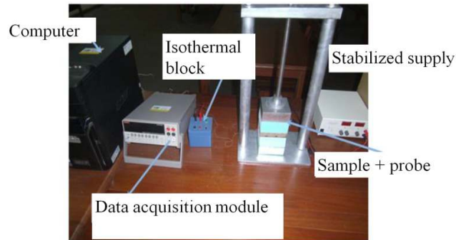
Figure 4: Experimental mechanism of thermal characterization of experience test
