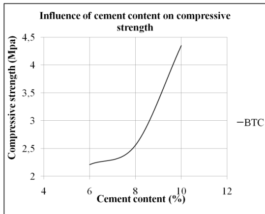
Figure 7: Influence of cement content on the resistances in compression
