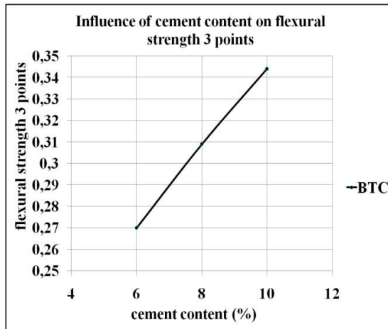
Figure 8: Influence of cement content on the resistances in flexion three points
