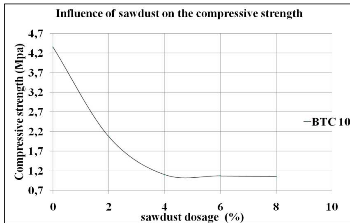
Figure 5: Influence of dosage of Afzelia sawdust on the resistance in compression
