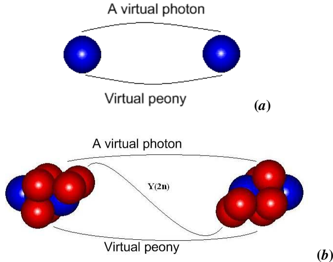
Fig. 5. A particle surrounded by virtual bosons: a - proton, b - ^9_3\text{Li} .
