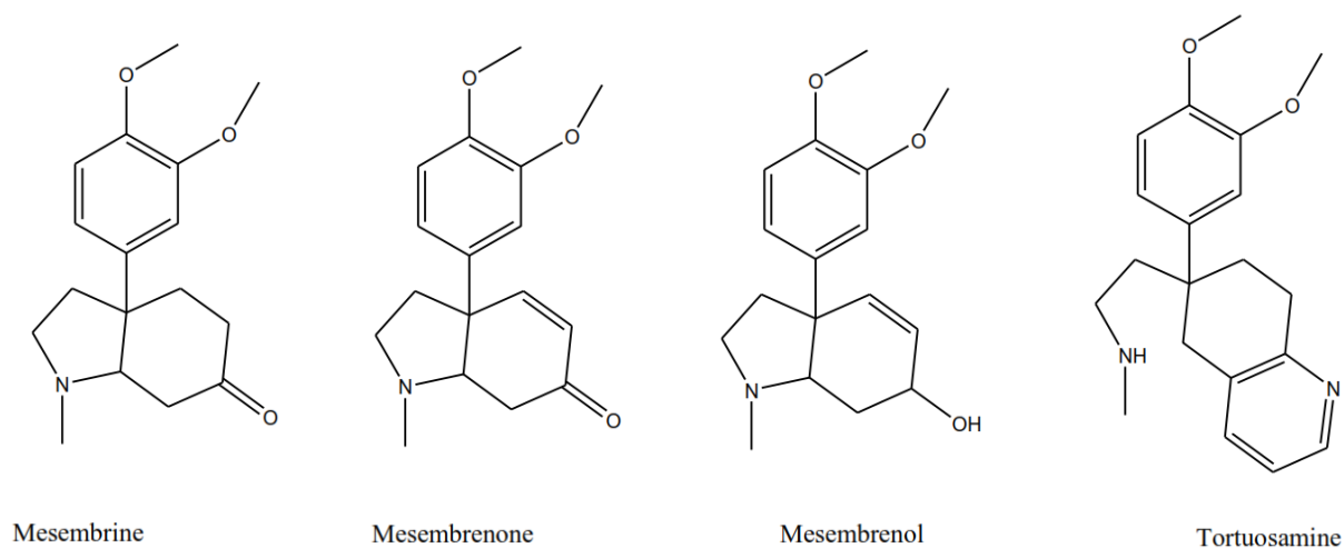
Figure 1: Structure of major chemical constituent's indole alkaloids in the Mesembryanthemum nodiflorum
