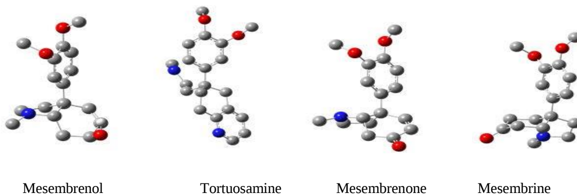
Figure 2: Optimized structure of major chemical constituent's indole alkaloids in the Mesembryanthemum nodiflorum plant without H-atom (for clarity)
