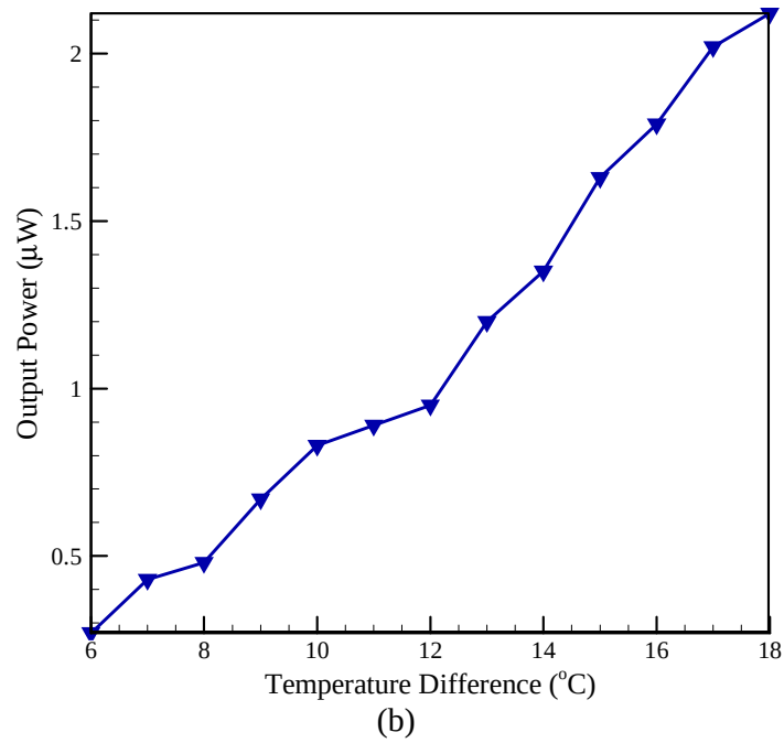
Fig. 11. (a) Open circuit voltage and short circuit current, (b) Output power with respect to the temperature difference.
