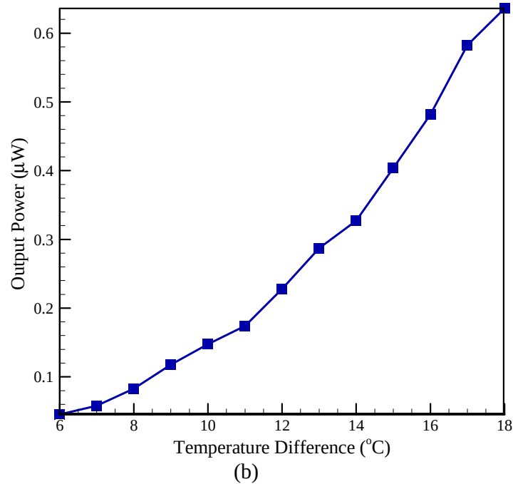
Fig. 4. (a) Open circuit voltage and short circuit current and (b) output power with respect to the temperature difference between the hot and ambient temperature for a single module.
