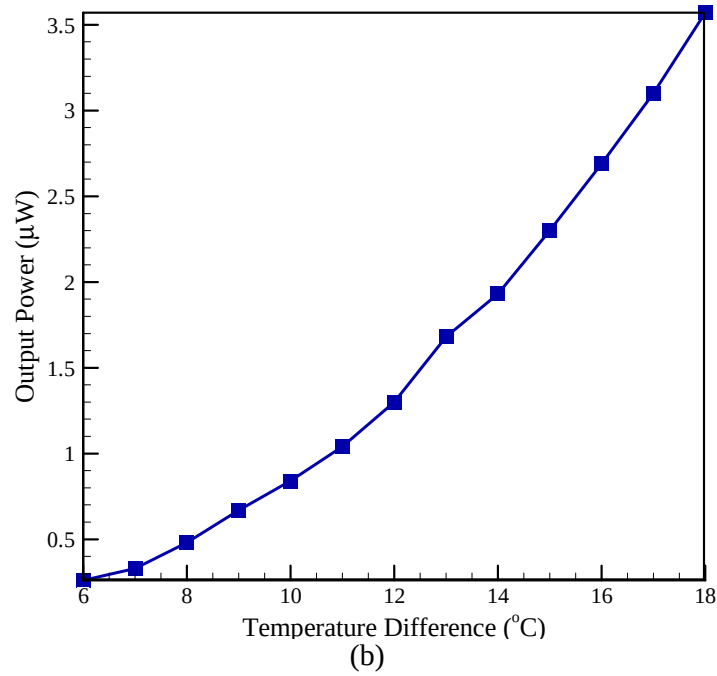
Fig. 7. (a) Open circuit voltage and short circuit current (b) Output power with respect to temperature for double modules.
