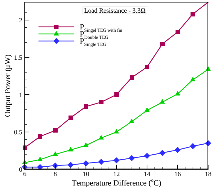
Fig. 13. Output power for three different configurations.
