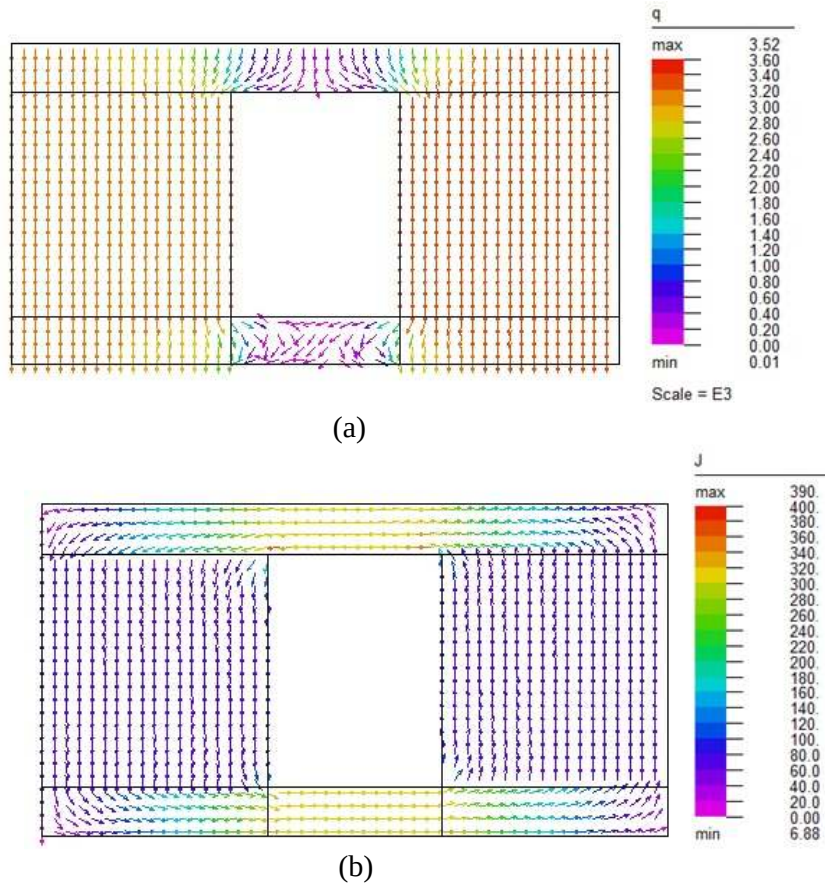
Fig. 19. (a) heat flow profile and (b) current density profile of a single TE module.
