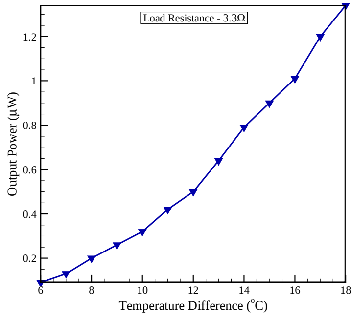
Fig. 8. (a) Load voltage and Load current, and (b) Output power with respect to temperature difference for double modules.
