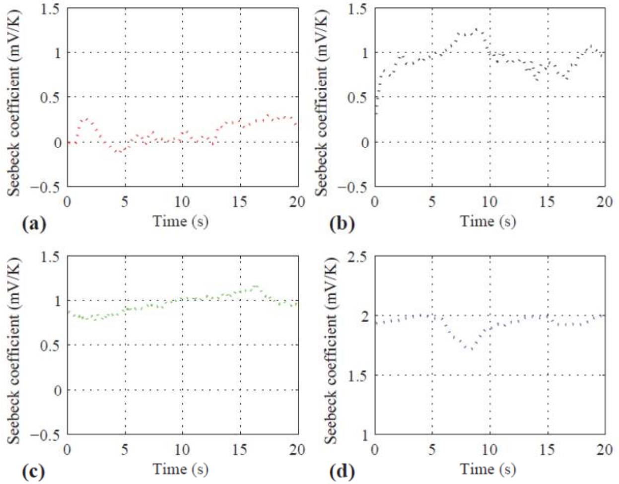
Figure 6 Seebeck coefficient measuring results of (a) SiAg, (b) SiAg-15, (c) SiAg-30, and (d) SiAg-60.
