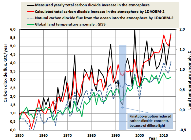
Fig. 9. The simulated fluxes from 1950 to 2013.
