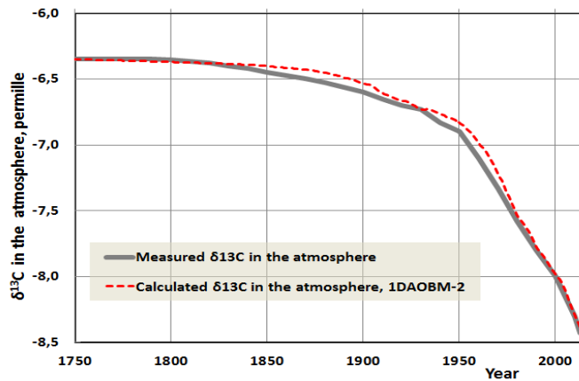
Fig. 10. The \delta^{13}\text{C} values according to the direct measurements and 1DAOBM-2.
