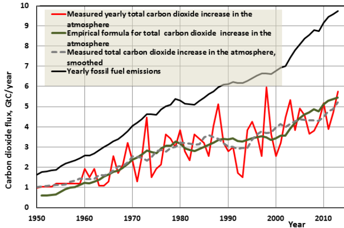
Fig. 3. The increase of the atmospheric \text{CO}_2 based on the linear empirical formula in comparison to the measured values.
