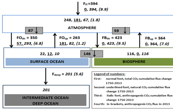
Fig. 5. The cumulative flux \text{CO}_2 flux changes values the between the reservoirs from 1750 to 2013, and cumulative changes of reservoirs from 1750 to 2013.
