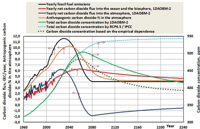
Fig. 8. The simulation results of the projection RCP4.5
