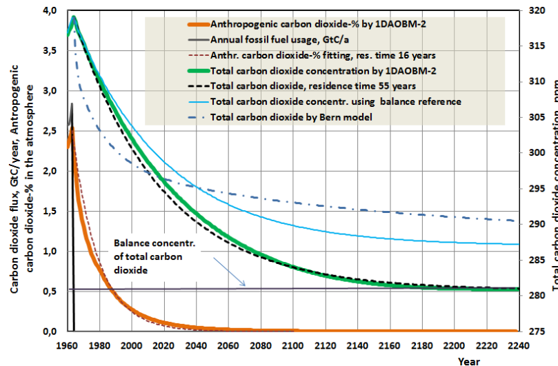
Fig.6. The simulated results of the fossil fuel change to zero \text{GtC yr}^{-1} in 1964 onward.
