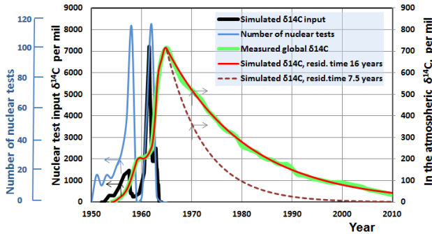
Fig. 2. The number of nuclear tests, the simulated δ 14 C input values, the measured δ 14 C values of radiocarbon and two simulated decay rates with 7.5 and 16 years residence times.
