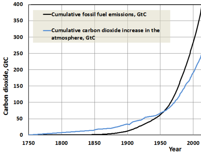
Fig. 4. The cumulative fossil fuel emissions and the cumulative \text{CO}_2 increase in the atmosphere from 1750 to 2015.
