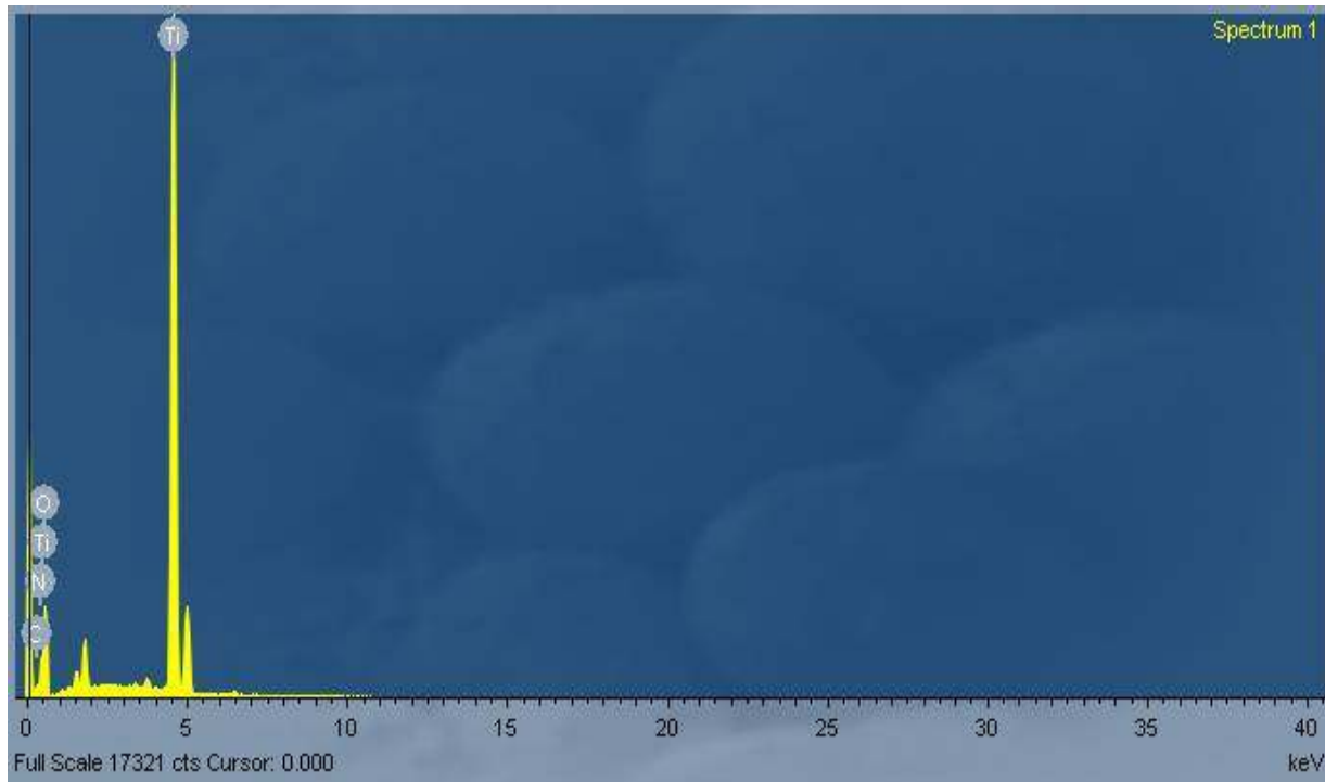
Fig. 3.4. EDX Image Showing the Elements Present in the TiO 2 Compound
