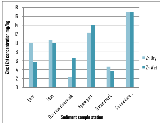
Fig 6. Zinc concentration in the sediment
