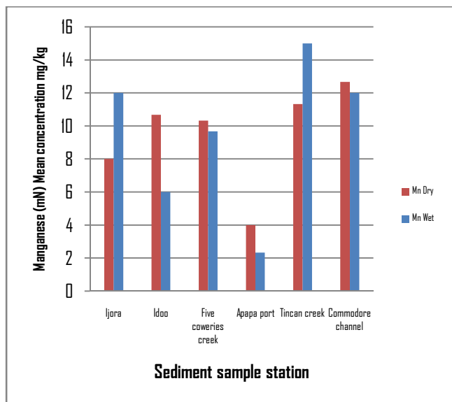
Fig 2. Manganese concentration in the sediment
