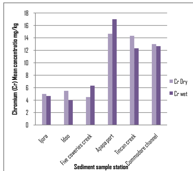
Fig 5. Chromium concentration in the sediment
