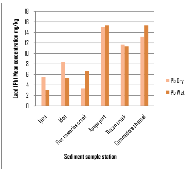
Fig 4. Lead concentration in the sediment
