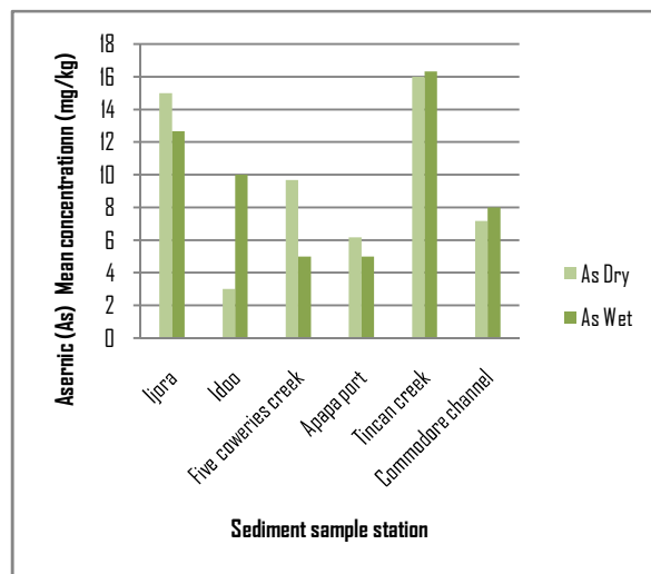
Fig 3. Arsenic concentration in the sediment
