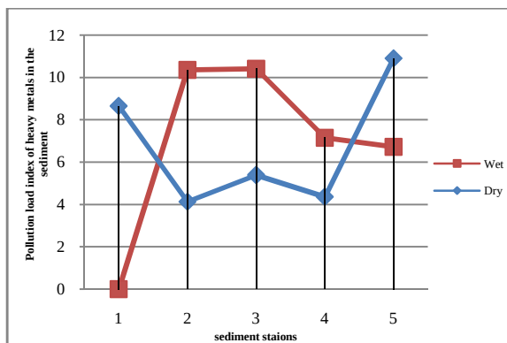
Fig 7. Pollution load index of heavy metals in the sediment of Lagos Lagoon
