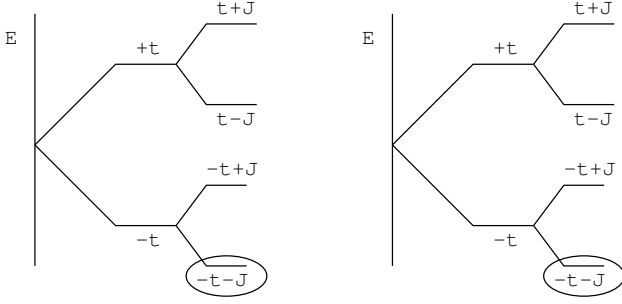
FIG. 7: Energy diagram for a single electron on an empty staggered ladder. If the staggered potential is large (large J ), the splitting J is more important than t . In the lowest state, there are only N/4 states. These are the same states as for a single one dimensional model where an electron moves in steps of two. If J \ll t (right) we still get the same lowest sector.
