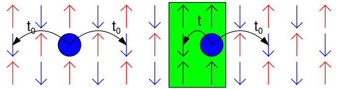
FIG. 5: One-dimensional example showing the reason for dynamical confinement . Outside the stripe, the hole moves in steps of two with an amplitude t_0 . Inside the stripe it can make a direct hop with amplitude t with t \gg t_0 .
