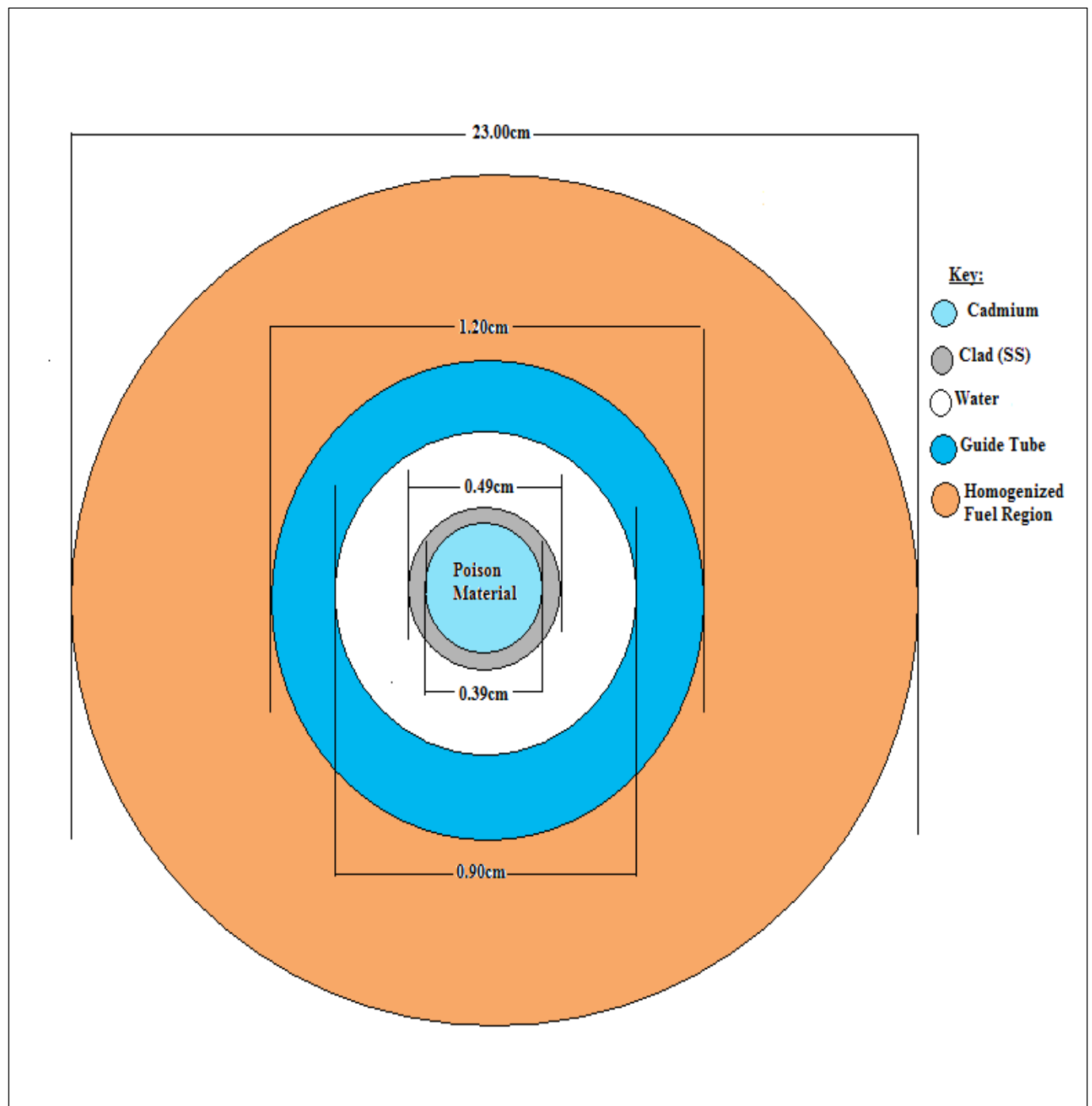
Figure 2: Description of the control model for NIRR-1 core.
