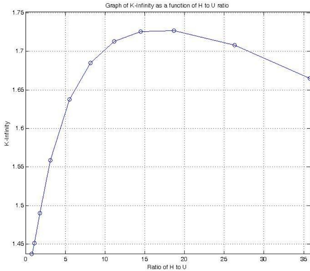
Figure 4: Plot of k-infinity as a function of H to U ratio for the LEU (19.75% \text{UO}_2 ) core
