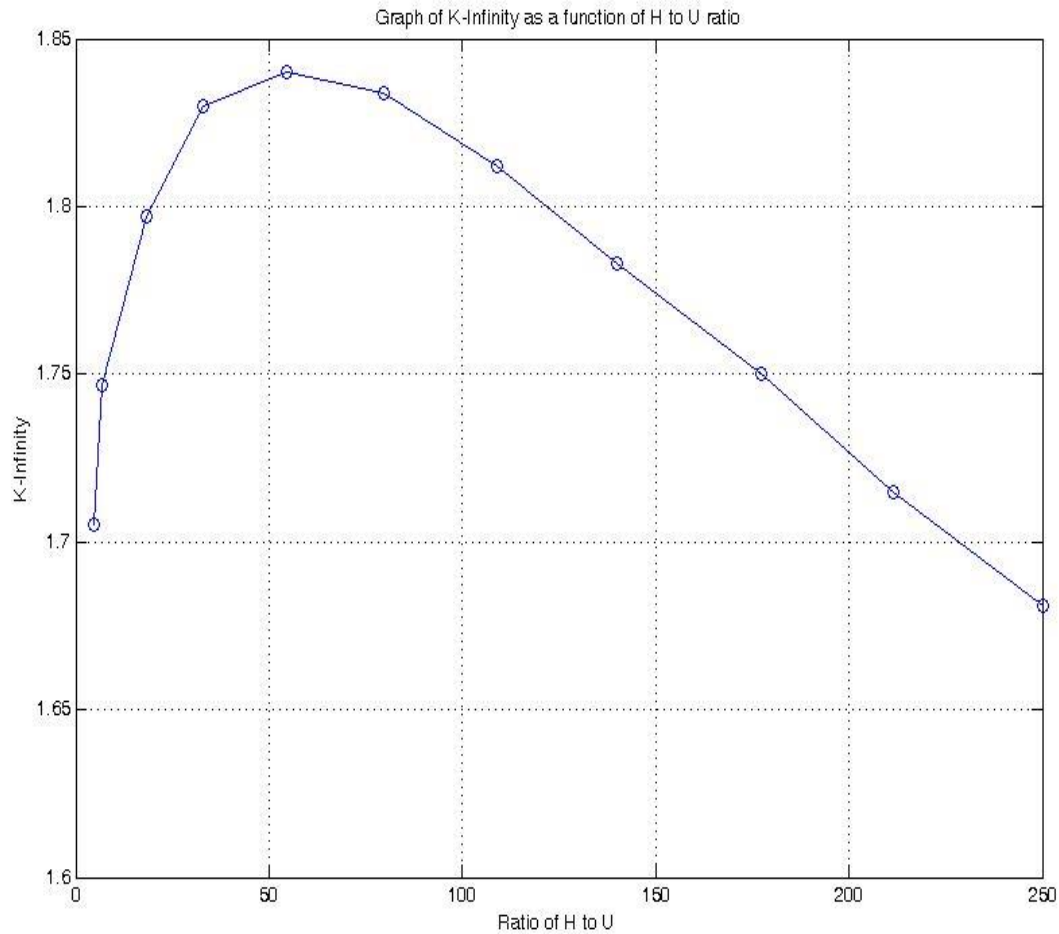
Figure 5: Plot of k-infinity as a function of H to U ratio for the HEU (90.2% UAl 4 ) core
