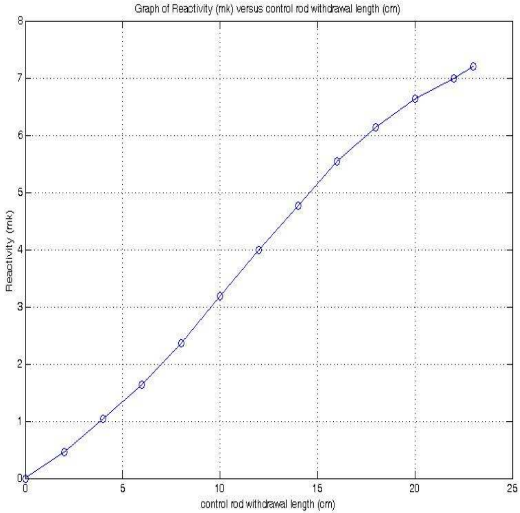
Figure 5: Reactivity (mk) versus control rod withdrawal length (cm) of active HEU (90.2% UAl 4 ) fuel region
