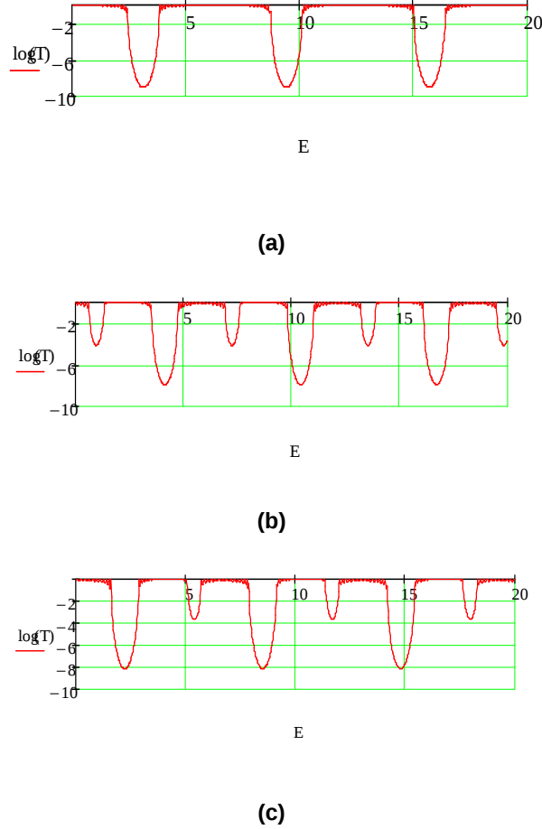
Fig. 3. Transmission spectra for the various values of the electrostatic potential U : U=0 , U=2 , U=4.5 for Fig. 3, a,b,c respectively, the other parameters: v_a=v_b=2 , d=1 , w=0.5
