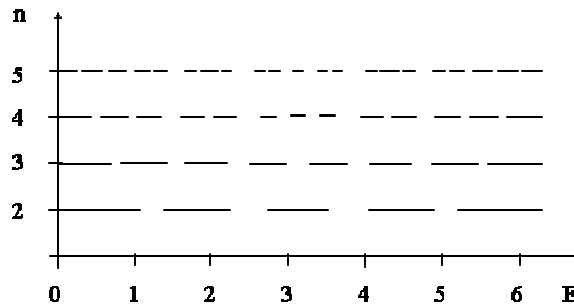
Fig. 2. Trace map for the initial Fibonacci generations, values of the parameters are as follows: d=1 , w=0.5 , v_a=1 , v_b=2
