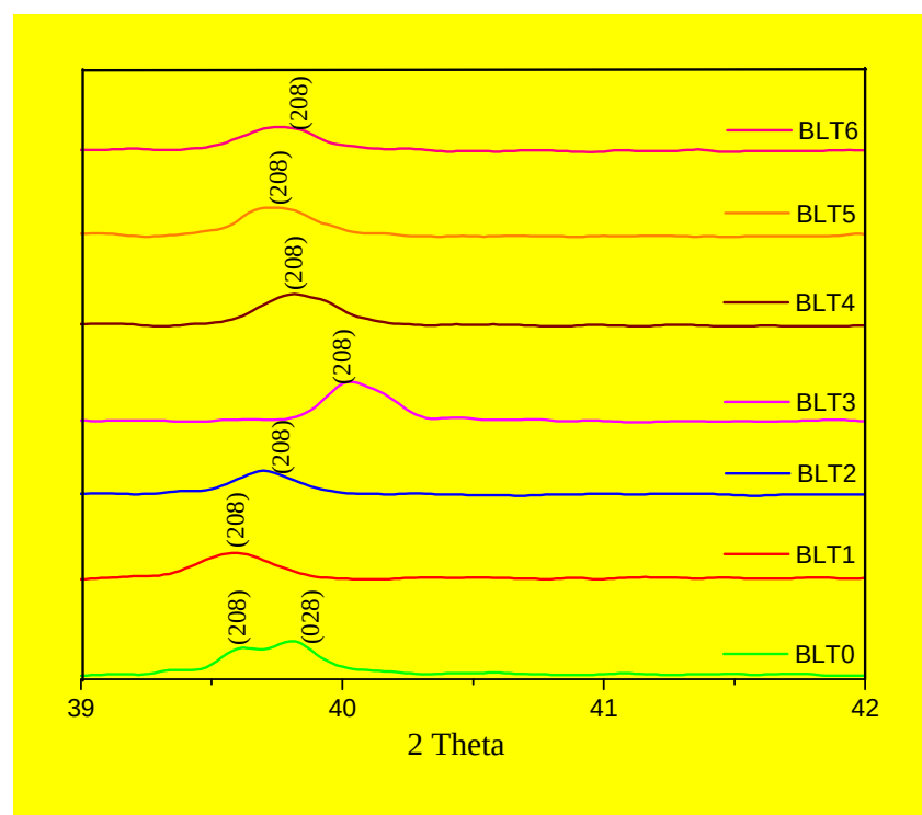
Fig. 4. Comparison of (h00), (h0l) and (0kl) planes with different La-doping.
