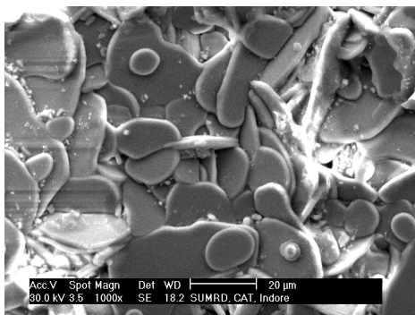
Fig. 6(a). Microstructure of BLT0.
