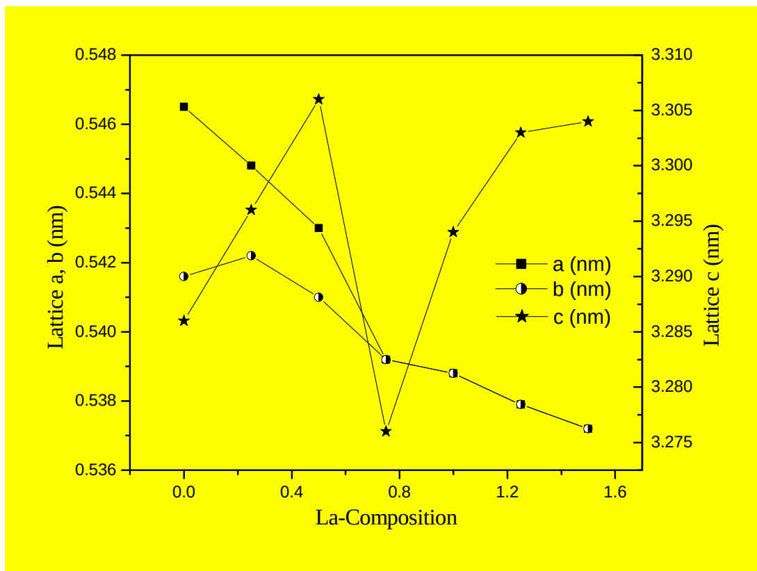
Fig. 5. Variation of lattice parameters with lanthanum doping in Bismuth titanate.
