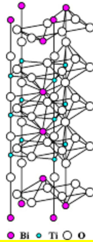
Fig. 1. Crystal structure of \text{Bi}_4\text{Ti}_3\text{O}_{12} [1].
