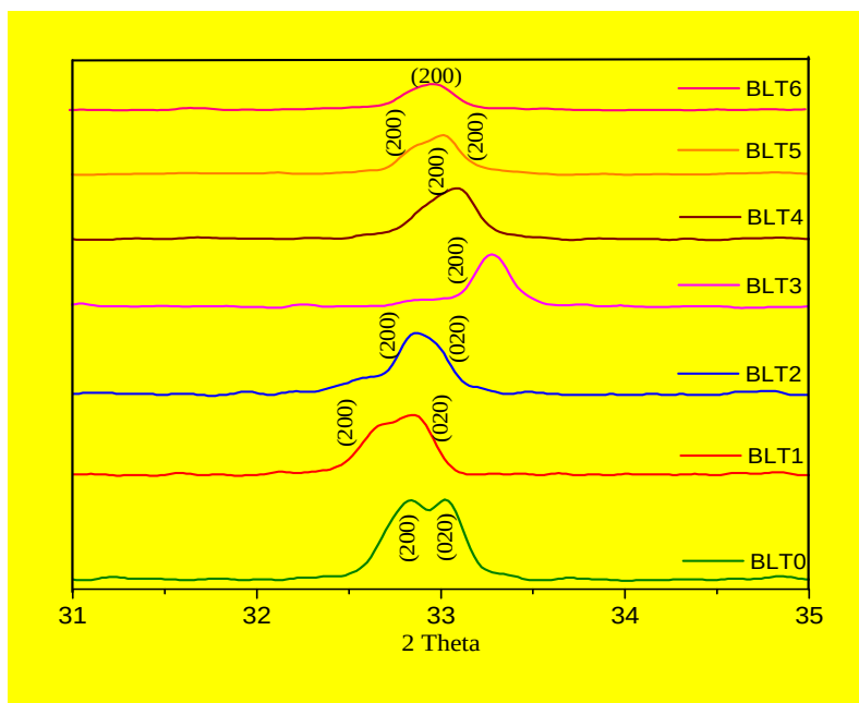
Fig. 3(b). Comparison of XRD patterns of \text{Bi}_{4-x}\text{La}_x\text{Ti}_3\text{O}_{12} ( x = 0 to 1.5 ) ceramics.
