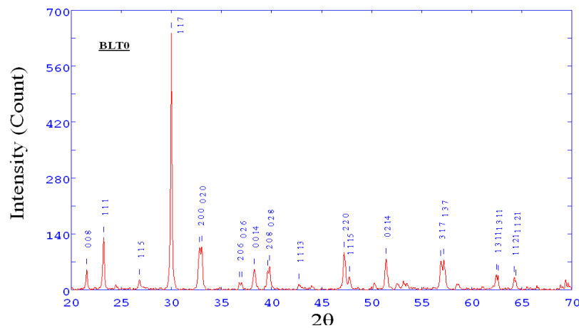
103 104 105 106 Fig. 3(a). Indexing of BLT0 using 'POWDER X' software.
