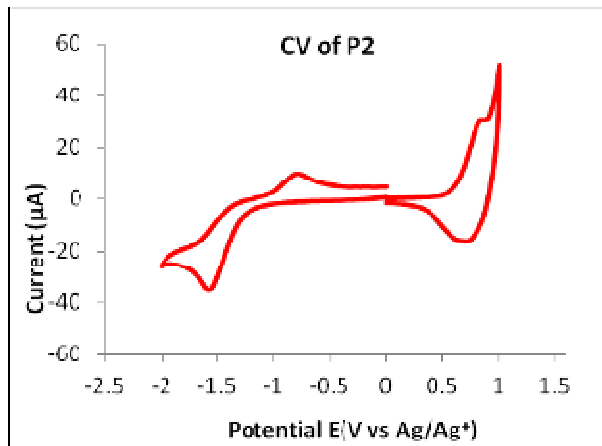
Figure 4: Cyclic voltammograms of P2 films cast on platinum disc (0.00314 cm 2 ) in tetrabutylammonium perchlorate/acetonitrile at 100mV/s
