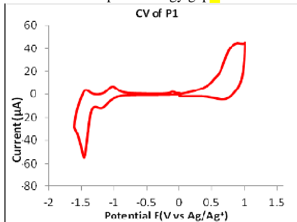
Figure 3: Cyclic voltammograms of P1 films cast on platinum disc (0.00314 cm 2 ) in tetrabutylammonium perchlorate/acetonitrile at 100mV/s
