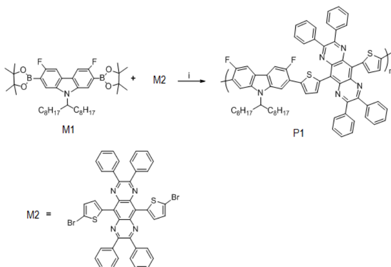
Scheme1: Preparation of polymer P1 (i) \text{Pd}(\text{AcO})_2 , tri-o-tolylphosphine, \text{NaHCO}_3 , THF
