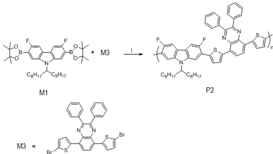
Scheme2: Preparation of polymer P2 (i) \text{Pd}(\text{AcO})_2 , tri-o-tolylphosphine, \text{NaHCO}_3 , THF
