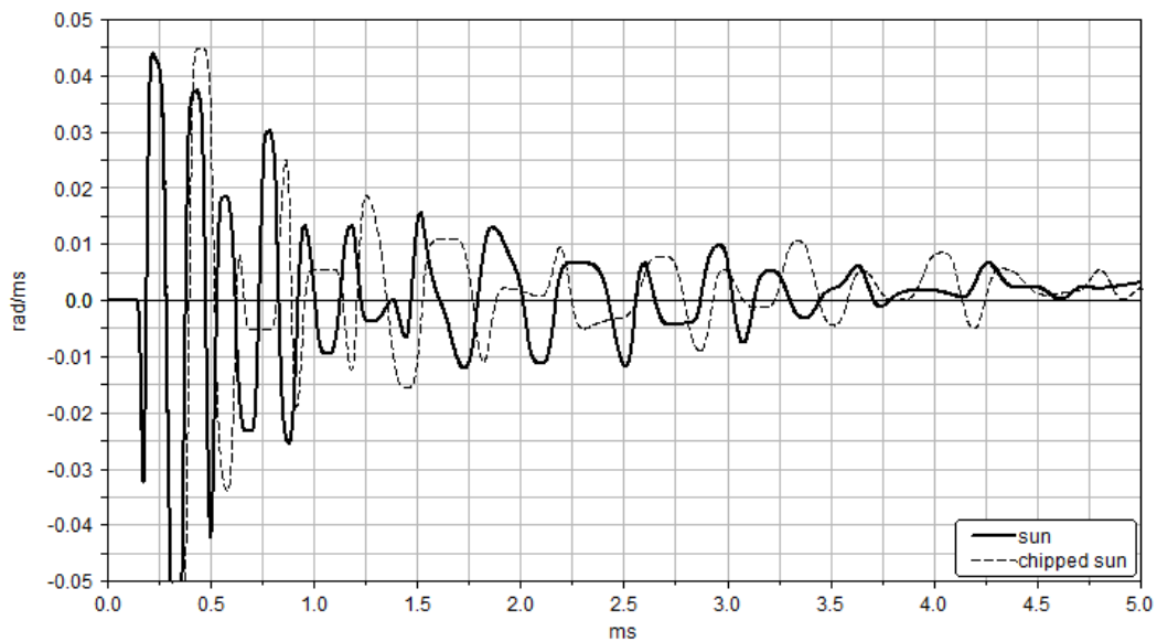
Fig.7. Sun angular velocity when the torque T_1 = 70.5 Nm is applied to the sun
