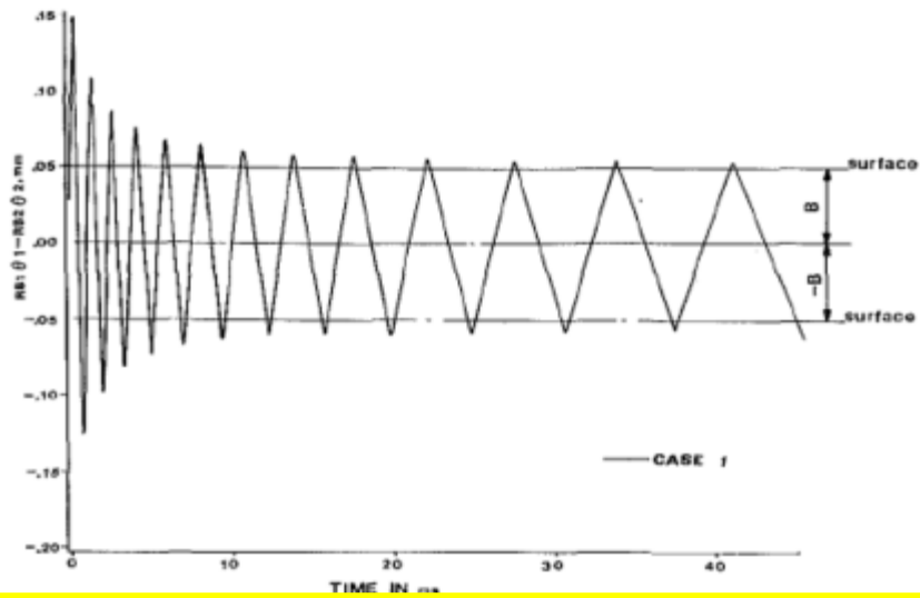
Fig.2. Relative displacement comparison. Free vibration with 50 rad/s pinion initial velocity; Top: simulation result; Bottom: ASME Journal publication [10]
