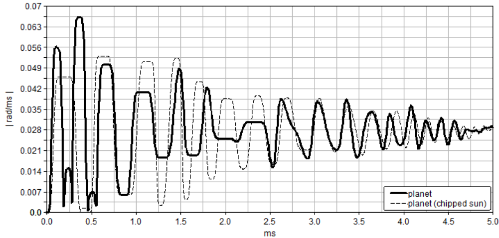
Fig.6. Angular velocities when constant angular velocity \omega_1 = 102.1 rad/s is applied to the sun
