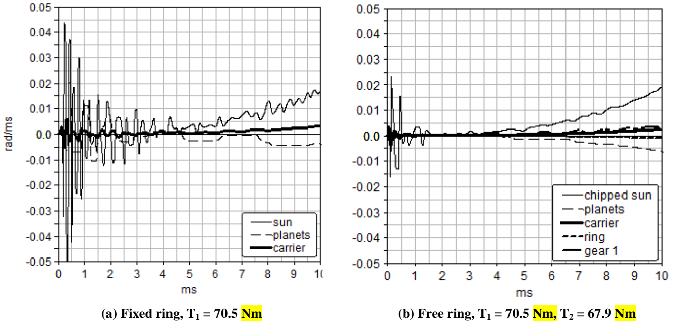
Fig.8. Angular velocity with applied step torques
