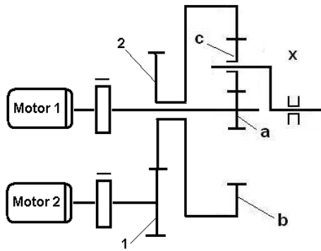
(a) Schematic
