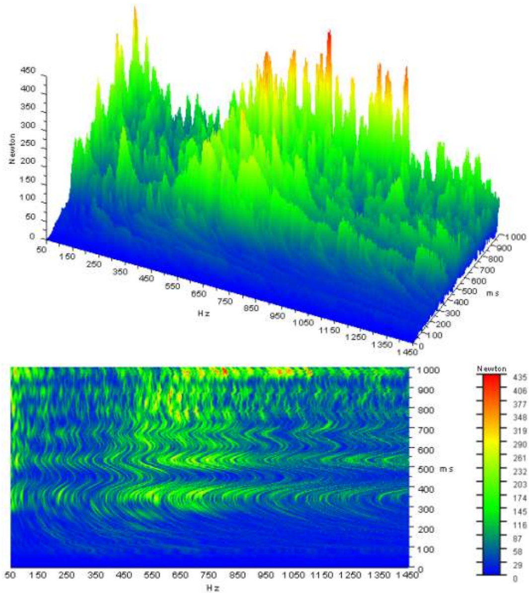
Fig.12. Three dimensional FFT of force magnitude in the fixed axis mesh for prescribed backlash and chipped sun with an exponential step angular velocity on both sun and gear 1
