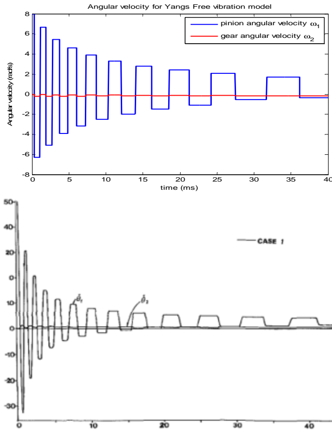
Fig.3. Angular velocities comparison. Free vibration with 50 rad/s pinion initial velocity; Top: simulation result; Bottom: ASME Journal publication [10]
