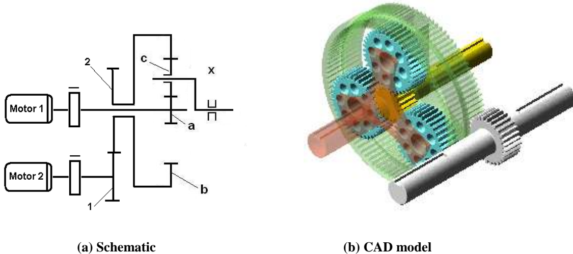
Fig.4. A differential planetary gear with two inputs and one output, the ring has both internal and external teeth
