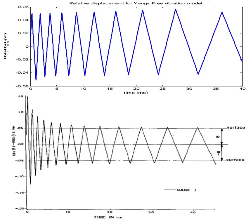
Fig. 8(a) Case 1: Relative displacement along the common normal
