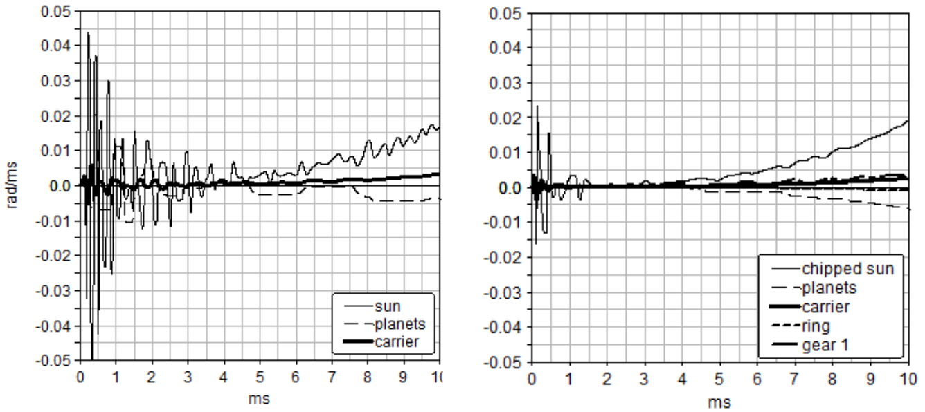
(a) Fixed ring, T_1 = 70.5 \text{ Nm}
