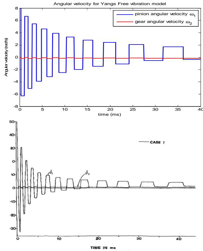
Fig. 8(c) Case 1: Angular velocities
