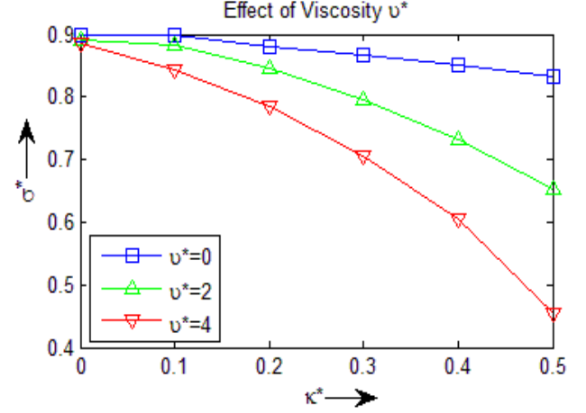
Fig. 4. The growth rate of instability is plotted against the dimensionless wave number k^* with variation in the viscosity \nu^* = 0, 2, 4 , with taking the values of \lambda^*, K_1^*, K_s^* and \tau^* as unity.
