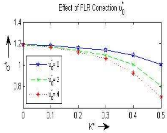
Fig. 8. The growth rate of instability is plotted against the dimensionless wave number k^* with variation in the finite Larmor radius \nu_0^* = 0, 2, 4 , with taking the values of K_s^*, \nu^*, \lambda^*, V^*, f^* and \tau^* as unity.
