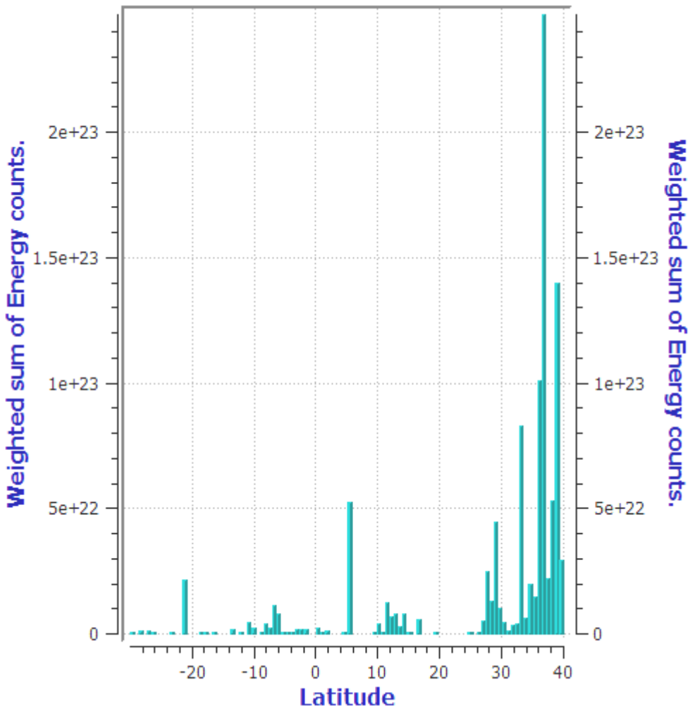
Figure 12: Weighted Sum of Seismic Energy against Latitude of Earthquakes in Africa 1974 – 2013
