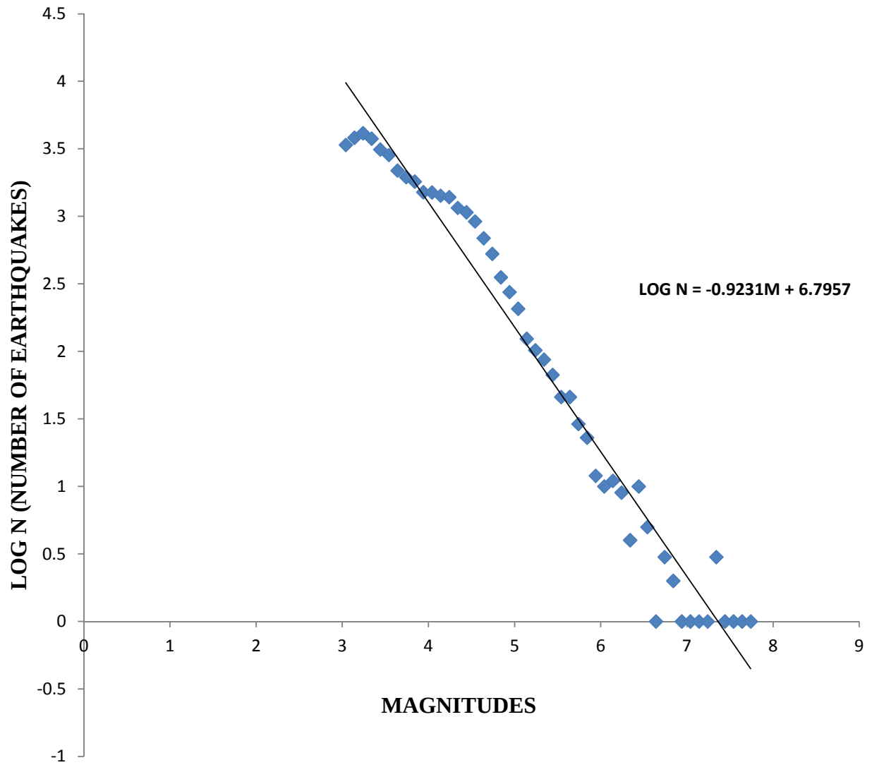
Figure 5: The Gutenberg – Richter Relation for the Northern Africa seismicity
