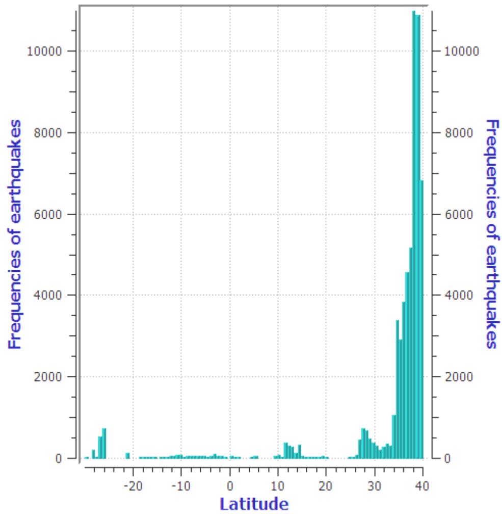
Figure 10: Frequency against Latitude of Earthquakes in Africa 1974 – 2013
