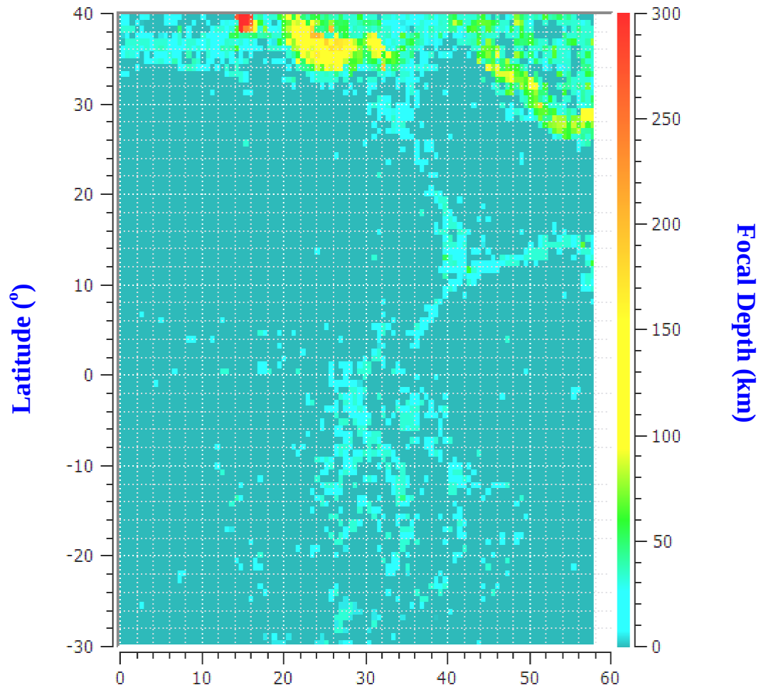
Figure 9: Focal Depth against Latitude and Longitude of Earthquakes in Africa 1974 – 2013
