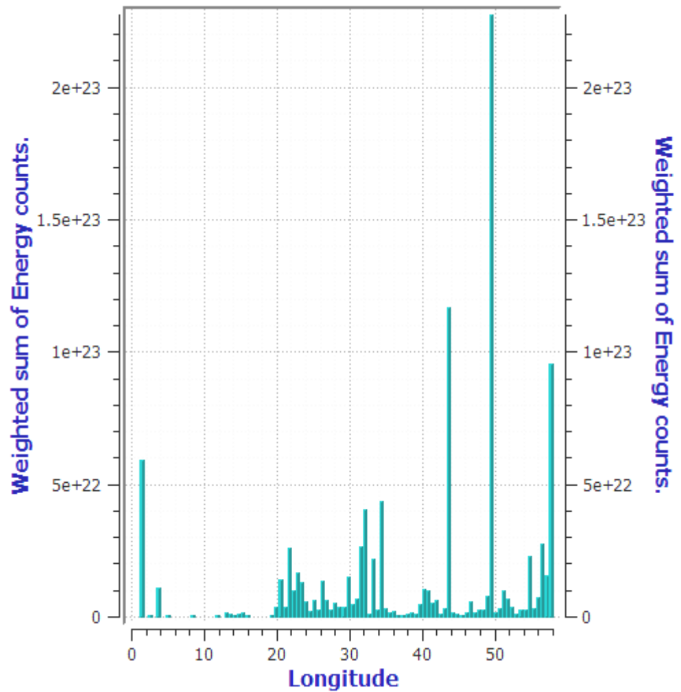
Figure 13: Weighted Sum of Seismic Energy against Longitude of Earthquakes in Africa 1974 – 2013
