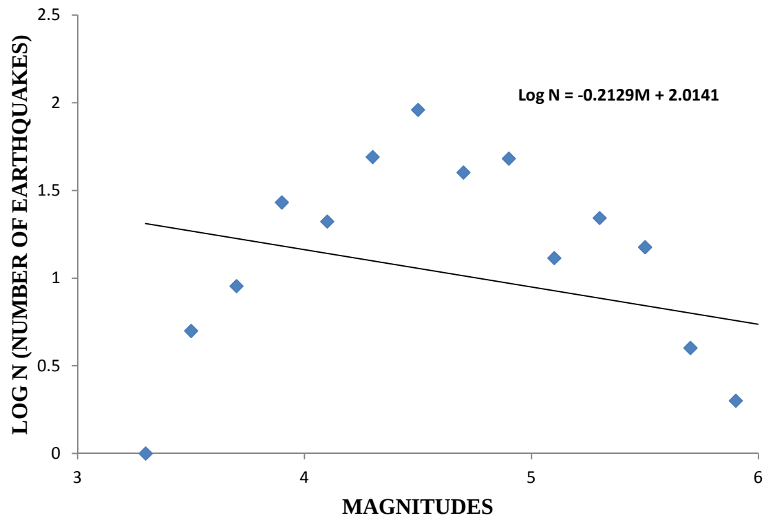
250 Figure 6: The Gutenberg – Richter Relation for the Eastern Africa seismicity
