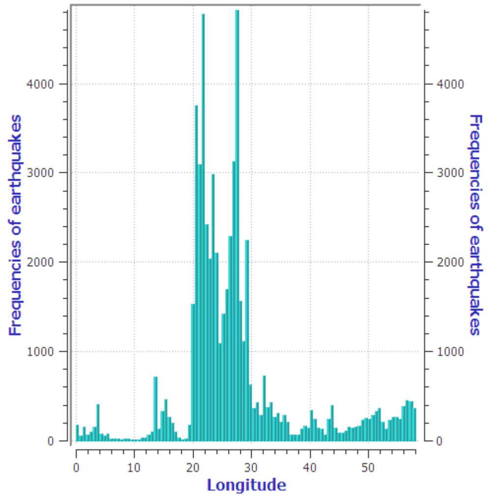
Figure 11: Frequency against Longitude of Earthquakes in Africa 1974 – 2013
