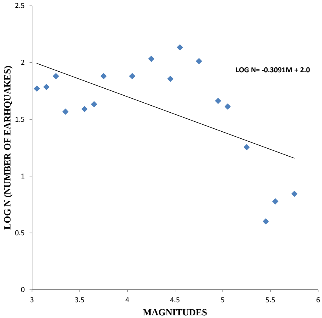
Figure 7: The Gutenberg – Richter Relation for the Southern Africa seismicity
