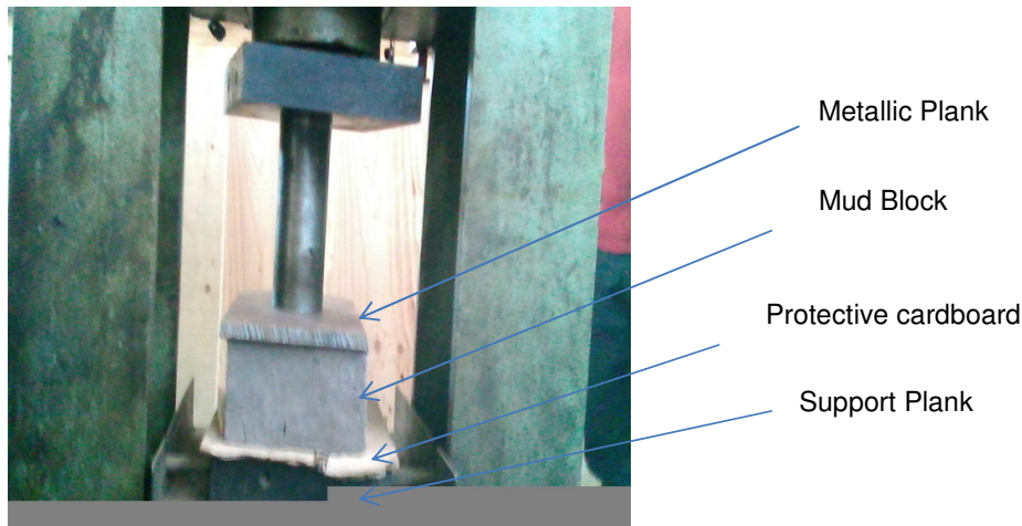
Figure 1 : Measuring Compressive Strength
