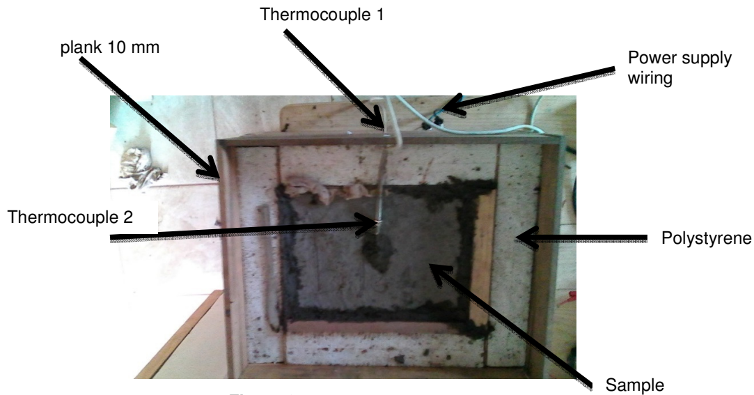
Figure 2: temperature measurement
