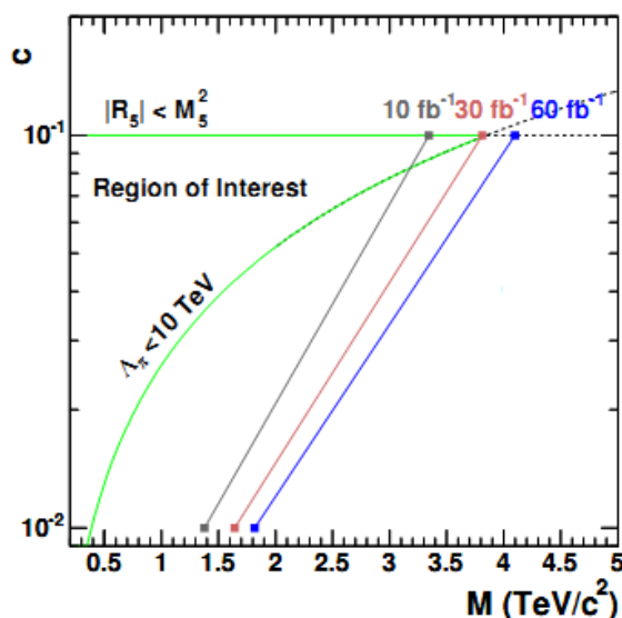
Fig. 2. Five \sigma discovery plane for graviton production as a function of the coupling parameter c and the graviton mass from [8]
