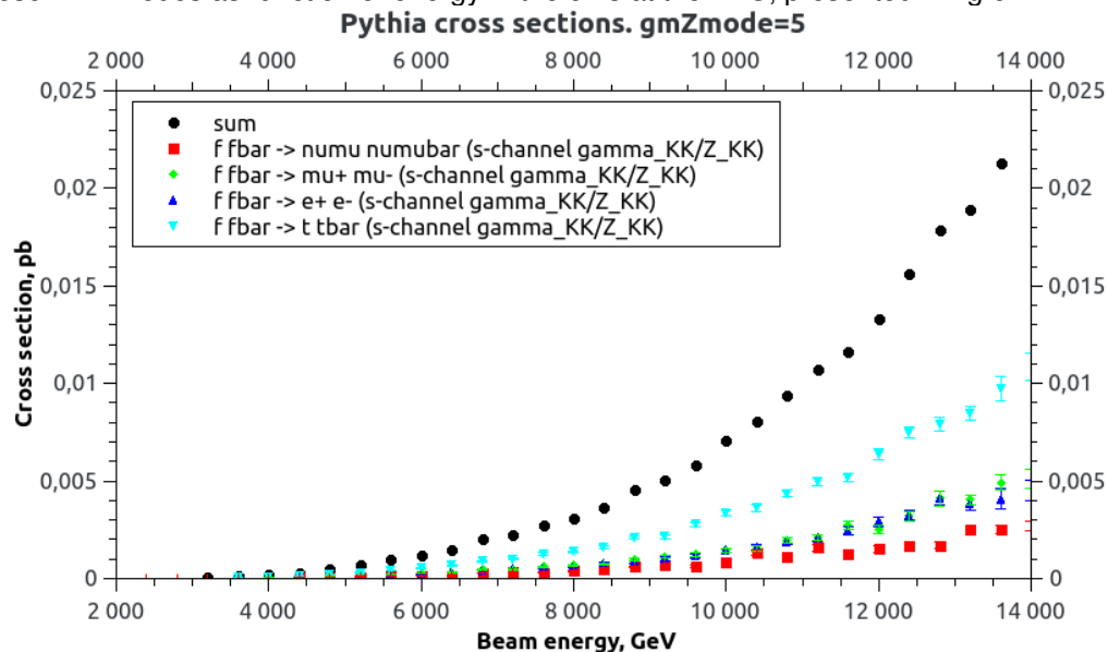
Fig. 6. Production cross section of KK vector boson as function of energy at the LHC with n=10 and M_c=4 TeV in the \text{TeV}^{-1} model
