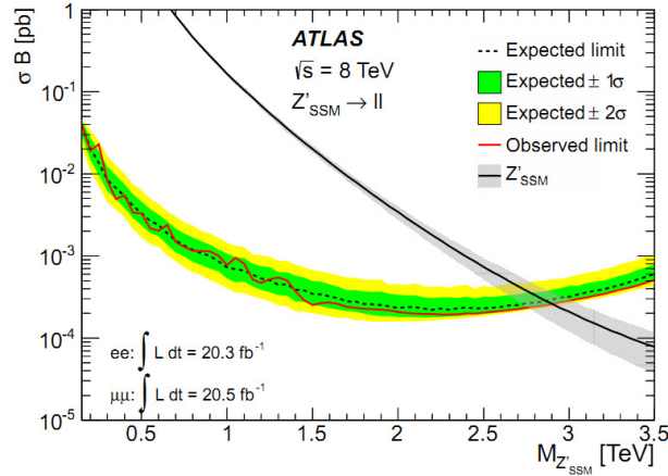
Fig. 10. 95% CL limits on the cross section \times branching ratio dependent on the resonance mass for the ATLAS [12] searches from [13].
