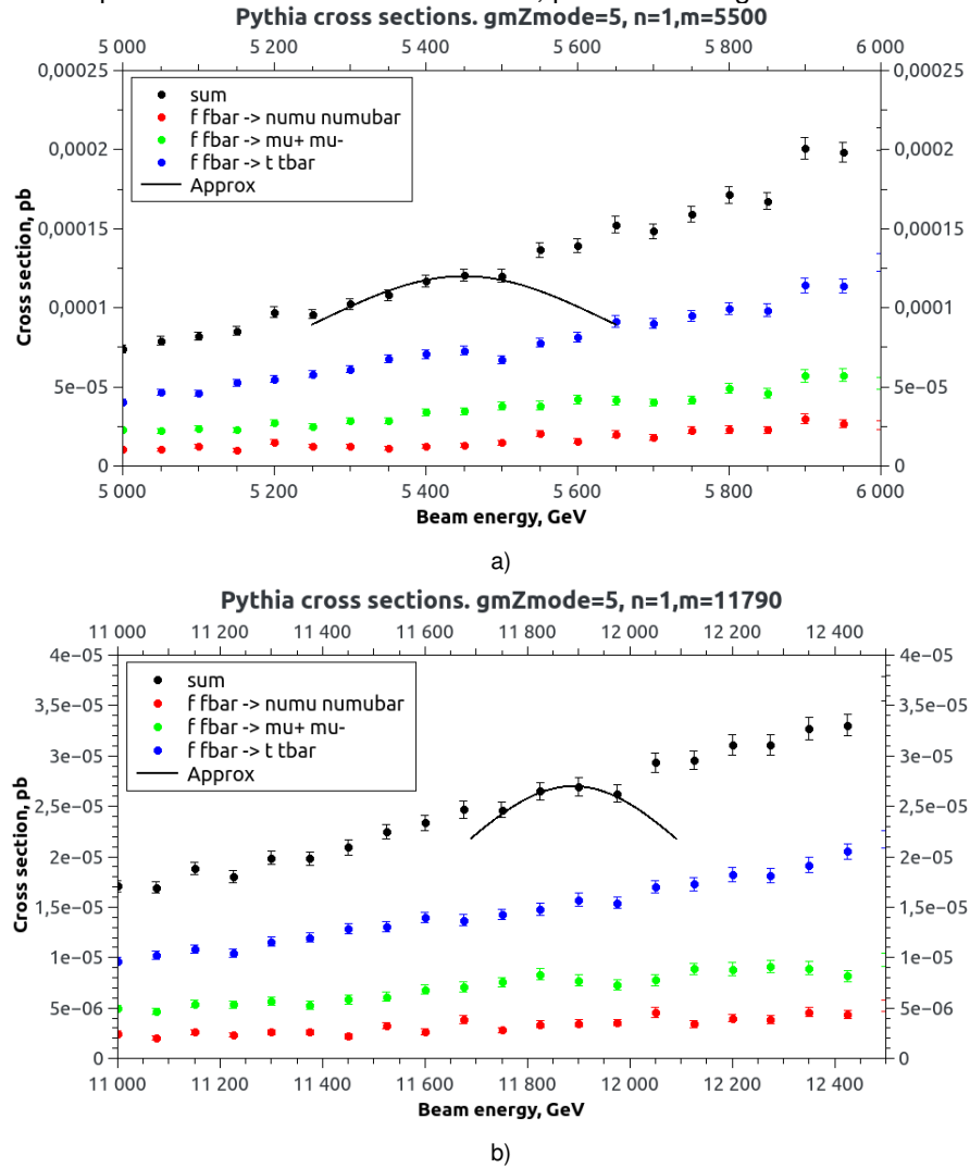
Fig. 7. KK vector boson production cross sections in the energy scale a) 5-6 TeV with parameters n=1 , M_c=5.5 TeV b) 11-12.4 TeV with parameters n=1 , M_c=11.79 TeV in the \text{TeV}^{-1} model
