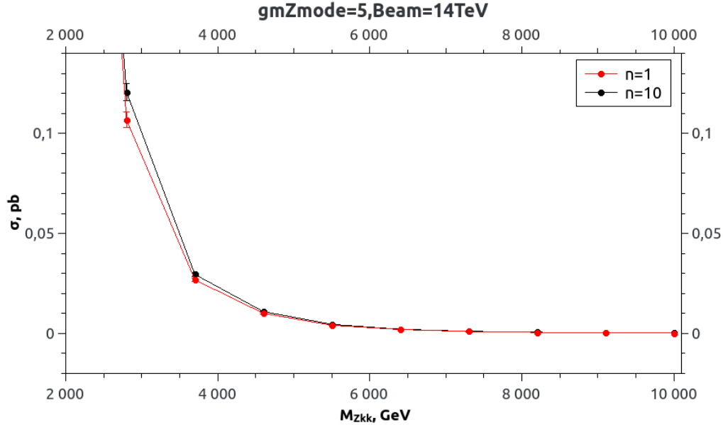
Fig. 8. The production cross section for the KK vector boson in the TeV-1 model
