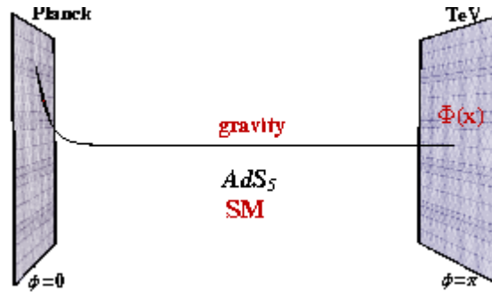
Fig. 1. Setup of the minimal Randall-Sundrum model
