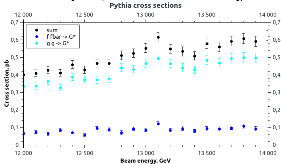
Fig. 5. KK graviton production cross sections in the energy scale 12-14 TeV at the LHC in the RS1 model
