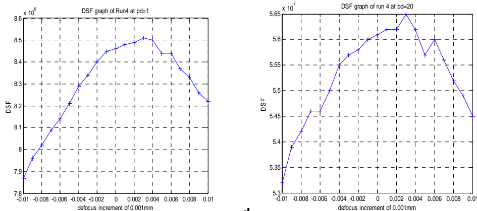
Figure 4 | Plot of DSF values against defocus increment 0.01mm for (a) pixel difference (k) of 1 (b) pixel difference (k) of 20. Defocus increment 0.001mm (c) pixel difference of 1 (d) pixel difference(k) of 20.
