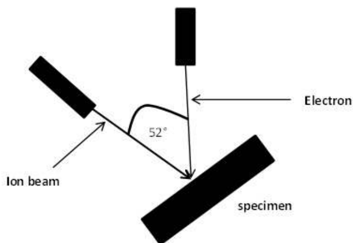
Figure 1 | A schematic diagram of the dual FIB/SEM. The angle between the FIB and SEM beams is 52^\circ , with the ion beam at 90^\circ to the specimen
