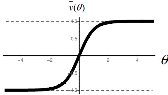
Figure 1.1. The graph of the normalized speed of the light source \bar{v}(\theta) = \frac{v(\theta)}{c} = th(\theta) (the black curve), \lim_{\theta \rightarrow \pm\infty} \bar{v}(\theta) = \pm 1 are the limit values of the normalized speed of the light source (the dashed lines).
